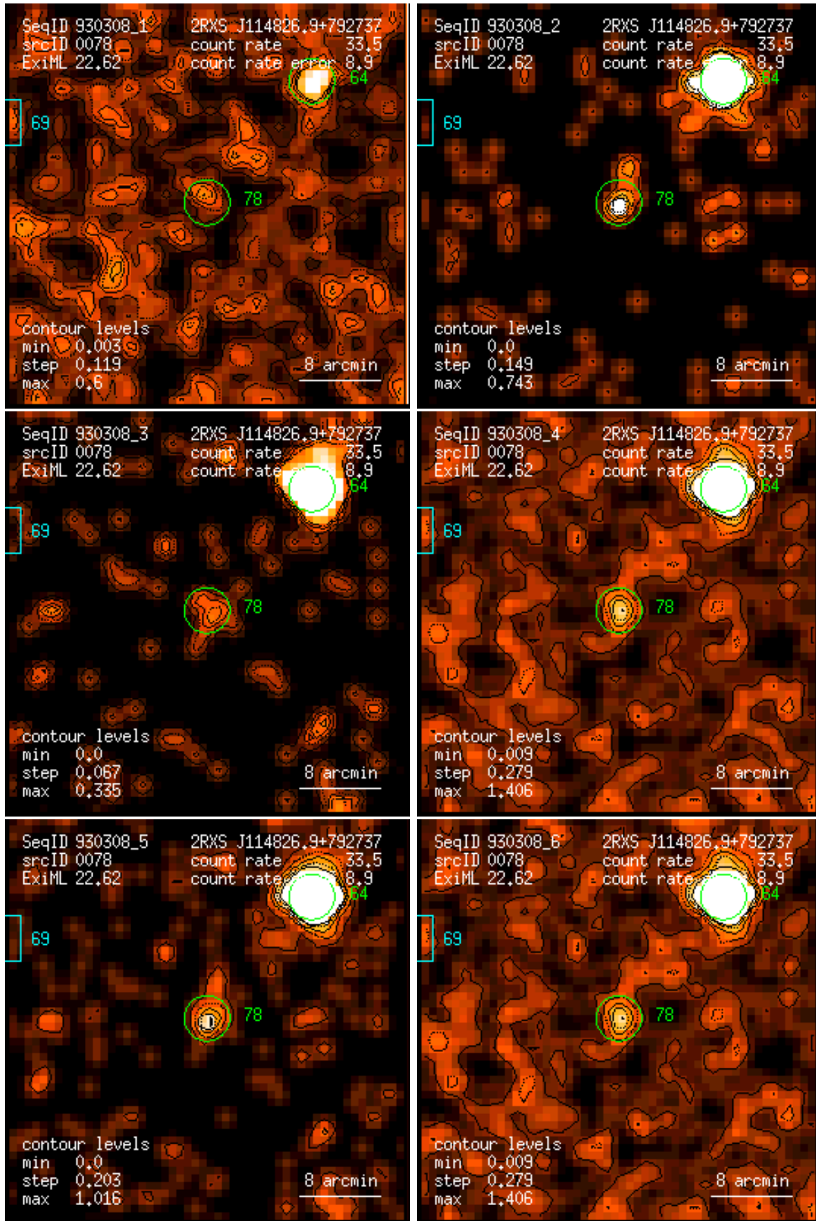
Figure 78: RASS 930308: detection 0078: band rate images, Gaussian filter: (1) PSPC channels 11 – 41, (2) 52 – 90, (3) 91 – 201, (4) 11 – 235, (5) 52 – 201, (6) 11 – 201. Broad band rates in counts/ks. Band rate contour levels in counts/ks/arcmin 2 .
