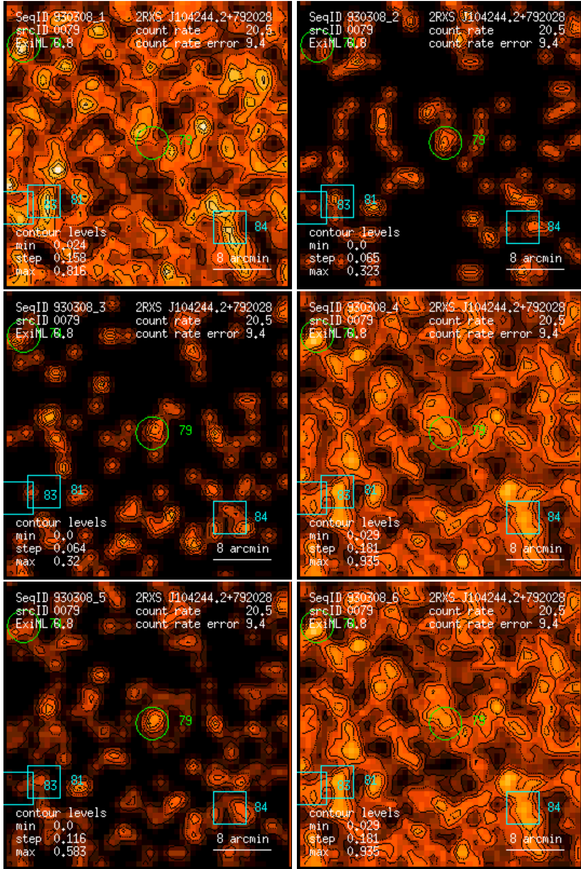
Figure 79: RASS 930308: detection 0079: band rate images, Gaussian filter: (1) PSPC channels 11 – 41, (2) 52 – 90, (3) 91 – 201, (4) 11 – 235, (5) 52 – 201, (6) 11 – 201. Broad band rates in counts/ks. Band rate contour levels in counts/ks/arcmin 2 .
