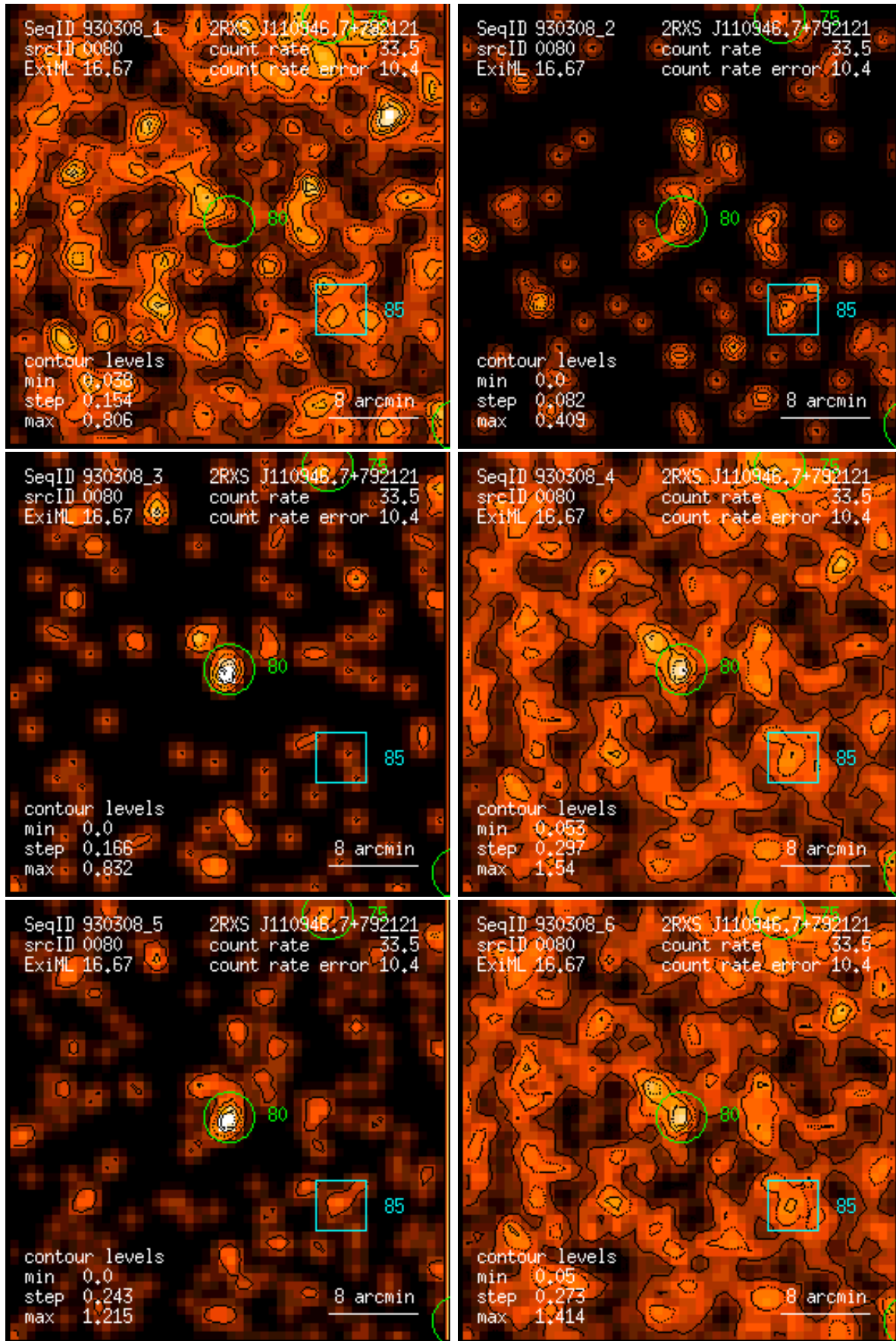
Figure 80: RASS 930308: detection 0080: band rate images, Gaussian filter: (1) PSPC channels 11 – 41, (2) 52 – 90, (3) 91 – 201, (4) 11 – 235, (5) 52 – 201, (6) 11 – 201. Broad band rates in counts/ks. Band rate contour levels in counts/ks/arcmin 2 .
