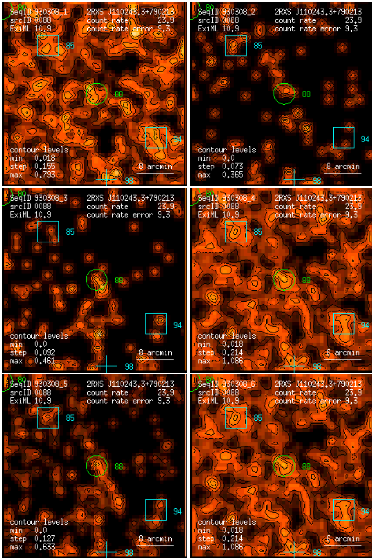
Figure 88: RASS 930308: detection 0088: band rate images, Gaussian filter: (1) PSPC channels 11 – 41, (2) 52 – 90, (3) 91 – 201, (4) 11 – 235, (5) 52 – 201, (6) 11 – 201. Broad band rates in counts/ks. Band rate contour levels in counts/ks/arcmin 2 .
