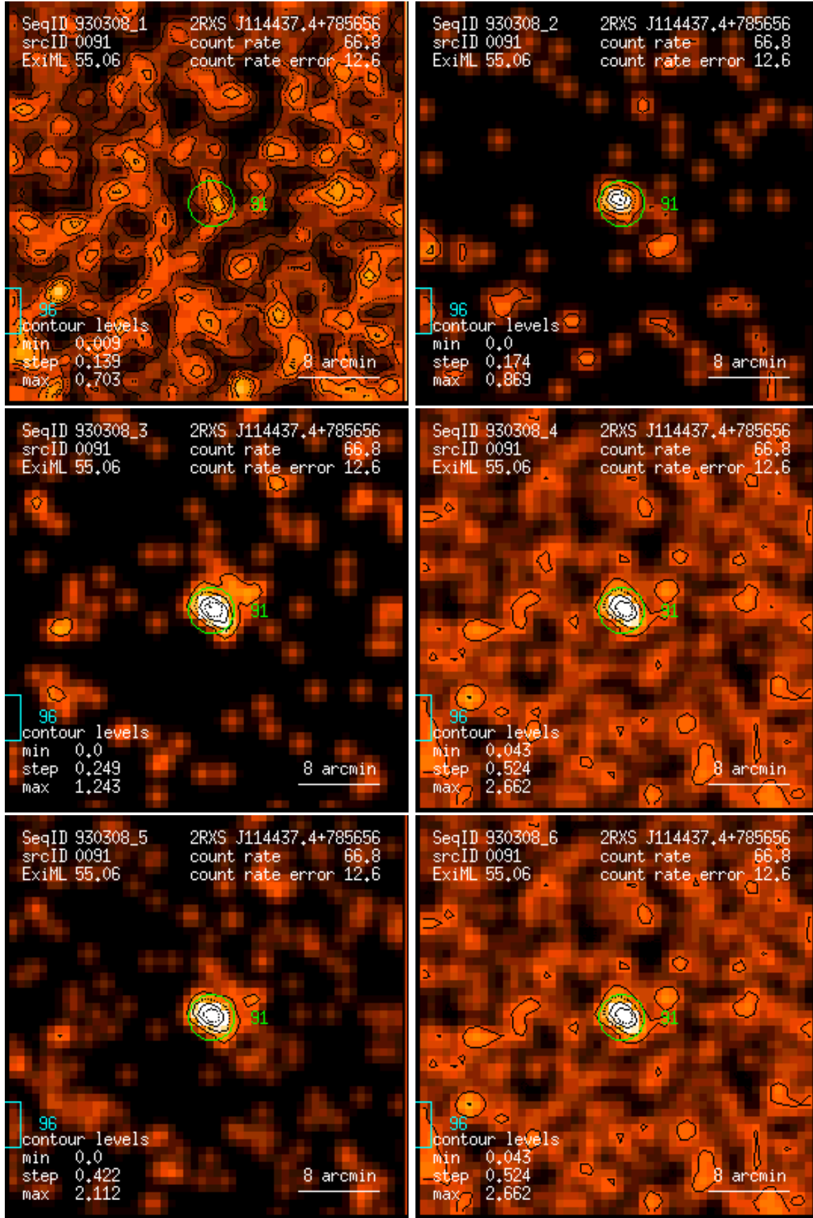
Figure 91: RASS 930308: detection 0091: band rate images, Gaussian filter: (1) PSPC channels 11 – 41, (2) 52 – 90, (3) 91 – 201, (4) 11 – 235, (5) 52 – 201, (6) 11 – 201. Broad band rates in counts/ks. Band rate contour levels in counts/ks/arcmin 2 .
