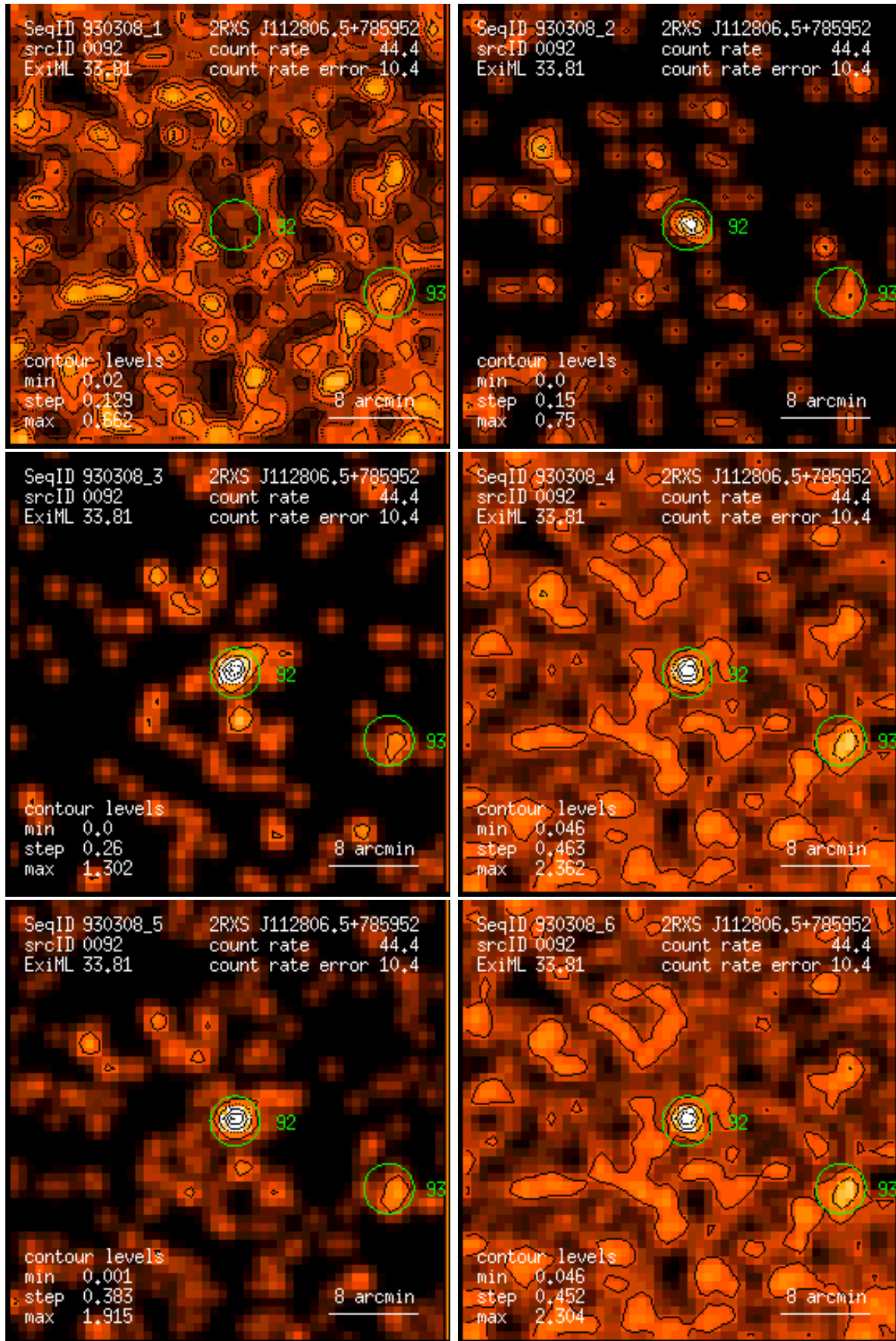
Figure 92: RASS 930308: detection 0092: band rate images, Gaussian filter: (1) PSPC channels 11 – 41, (2) 52 – 90, (3) 91 – 201, (4) 11 – 235, (5) 52 – 201, (6) 11 – 201. Broad band rates in counts/ks. Band rate contour levels in counts/ks/arcmin 2 .
