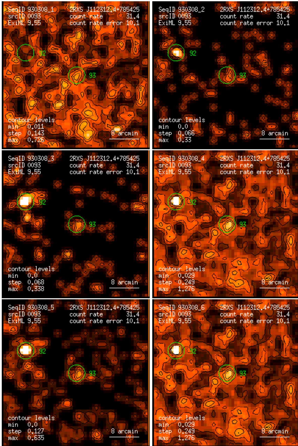
Figure 93: RASS 930308: detection 0093: band rate images, Gaussian filter: (1) PSPC channels 11 – 41, (2) 52 – 90, (3) 91 – 201, (4) 11 – 235, (5) 52 – 201, (6) 11 – 201. Broad band rates in counts/ks. Band rate contour levels in counts/ks/arcmin 2 .
