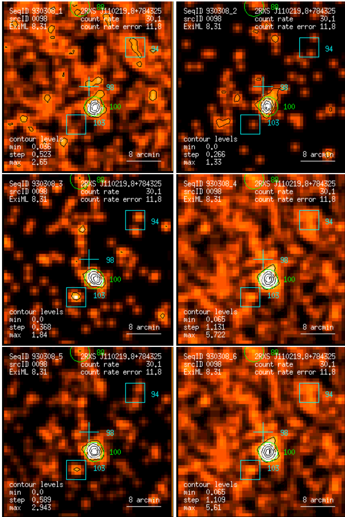
Figure 98: RASS 930308: detection 0098: band rate images, Gaussian filter: (1) PSPC channels 11 – 41, (2) 52 – 90, (3) 91 – 201, (4) 11 – 235, (5) 52 – 201, (6) 11 – 201. Broad band rates in counts/ks. Band rate contour levels in counts/ks/arcmin 2 .
