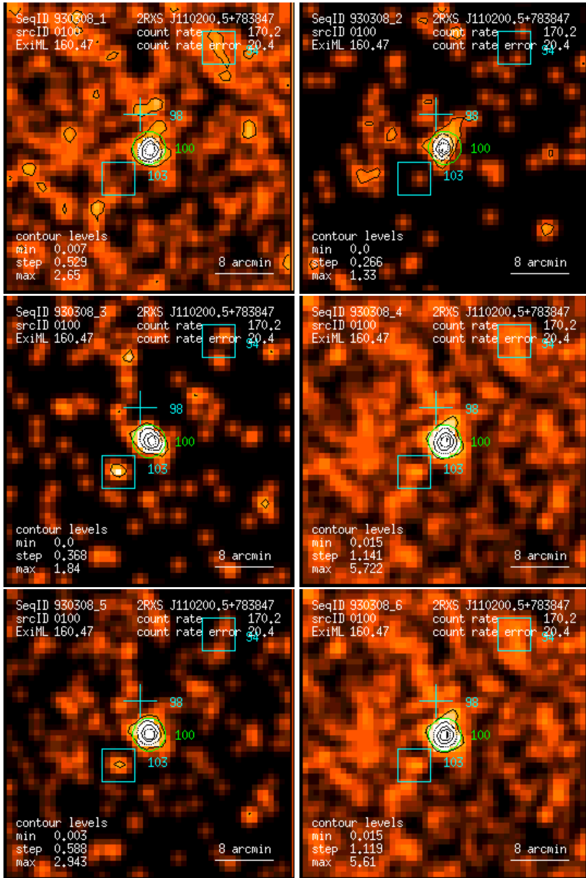
Figure 100: RASS 930308: detection 0100: band rate images, Gaussian filter: (1) PSPC channels 11 – 41, (2) 52 – 90, (3) 91 – 201, (4) 11 – 235, (5) 52 – 201, (6) 11 – 201. Broad band rates in counts/ks. Band rate contour levels in counts/ks/arcmin 2 .
