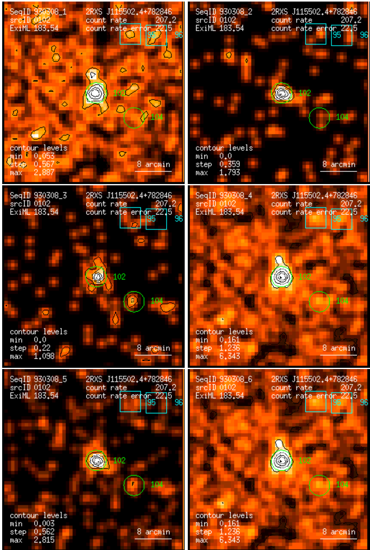
Figure 102: RASS 930308: detection 0102: band rate images, Gaussian filter: (1) PSPC channels 11 – 41, (2) 52 – 90, (3) 91 – 201, (4) 11 – 235, (5) 52 – 201, (6) 11 – 201. Broad band rates in counts/ks. Band rate contour levels in counts/ks/arcmin 2 .
