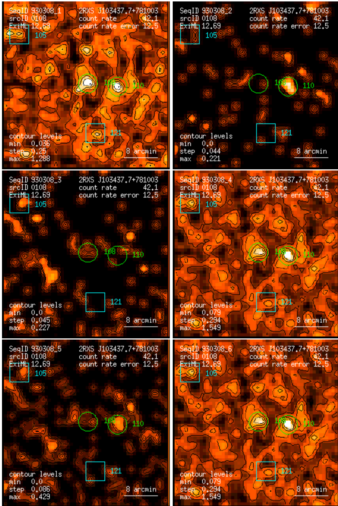
Figure 108: RASS 930308: detection 0108: band rate images, Gaussian filter: (1) PSPC channels 11 – 41, (2) 52 – 90, (3) 91 – 201, (4) 11 – 235, (5) 52 – 201, (6) 11 – 201. Broad band rates in counts/ks. Band rate contour levels in counts/ks/arcmin 2 .
