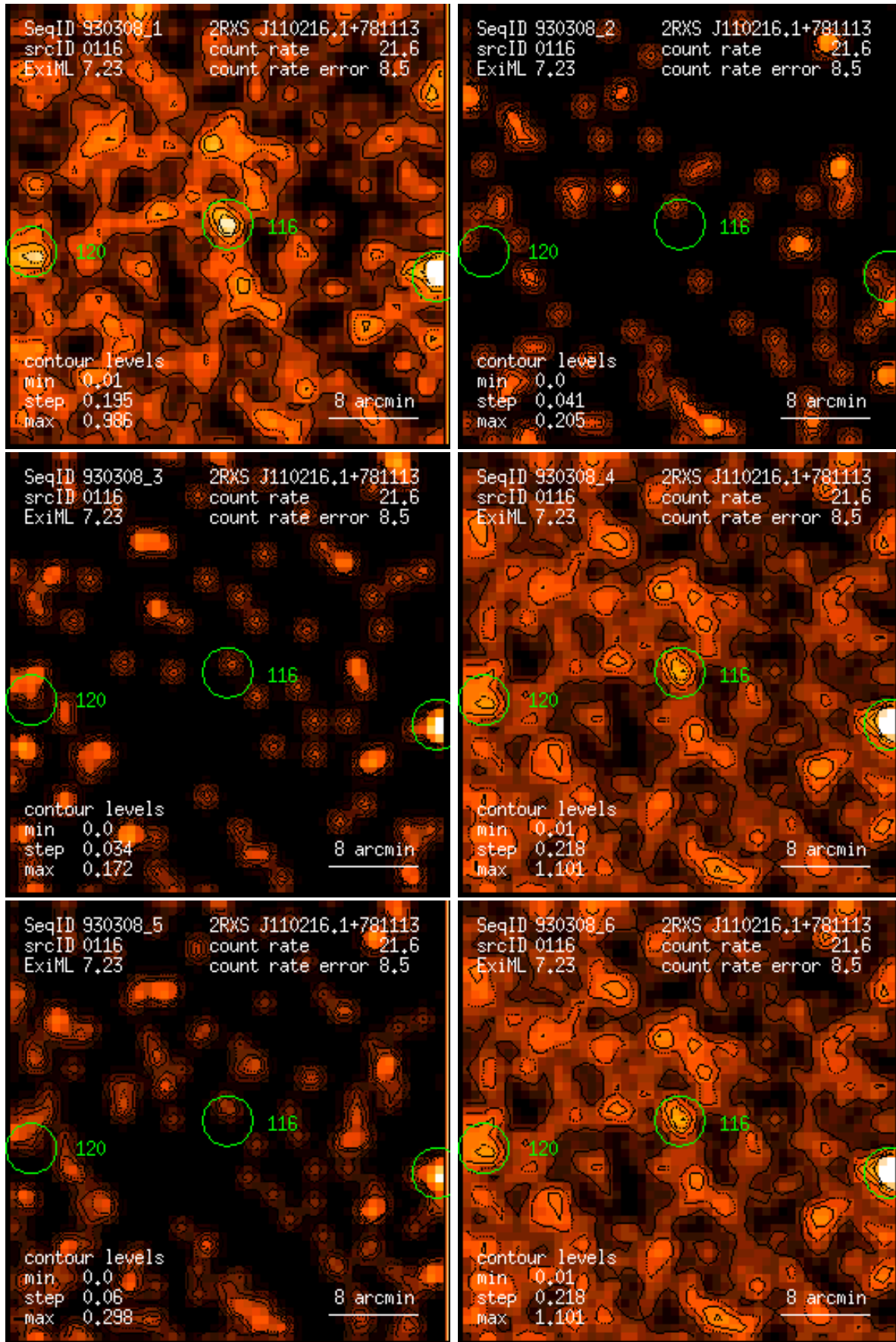
Figure 116: RASS 930308: detection 0116: band rate images, Gaussian filter: (1) PSPC channels 11 – 41, (2) 52 – 90, (3) 91 – 201, (4) 11 – 235, (5) 52 – 201, (6) 11 – 201. Broad band rates in counts/ks. Band rate contour levels in counts/ks/arcmin 2 .
