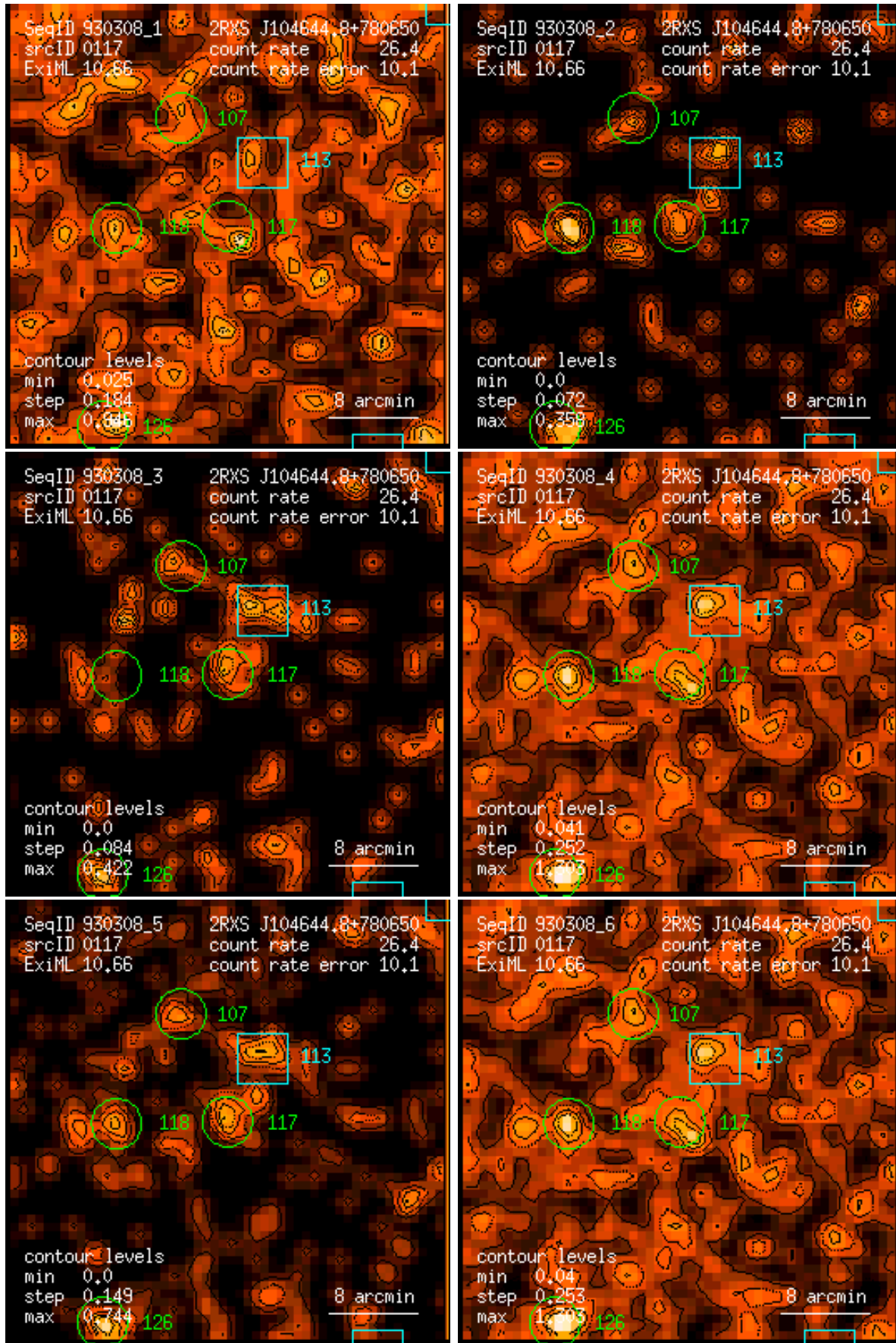
Figure 117: RASS 930308: detection 0117: band rate images, Gaussian filter: (1) PSPC channels 11 – 41, (2) 52 – 90, (3) 91 – 201, (4) 11 – 235, (5) 52 – 201, (6) 11 – 201. Broad band rates in counts/ks. Band rate contour levels in counts/ks/arcmin 2 .
