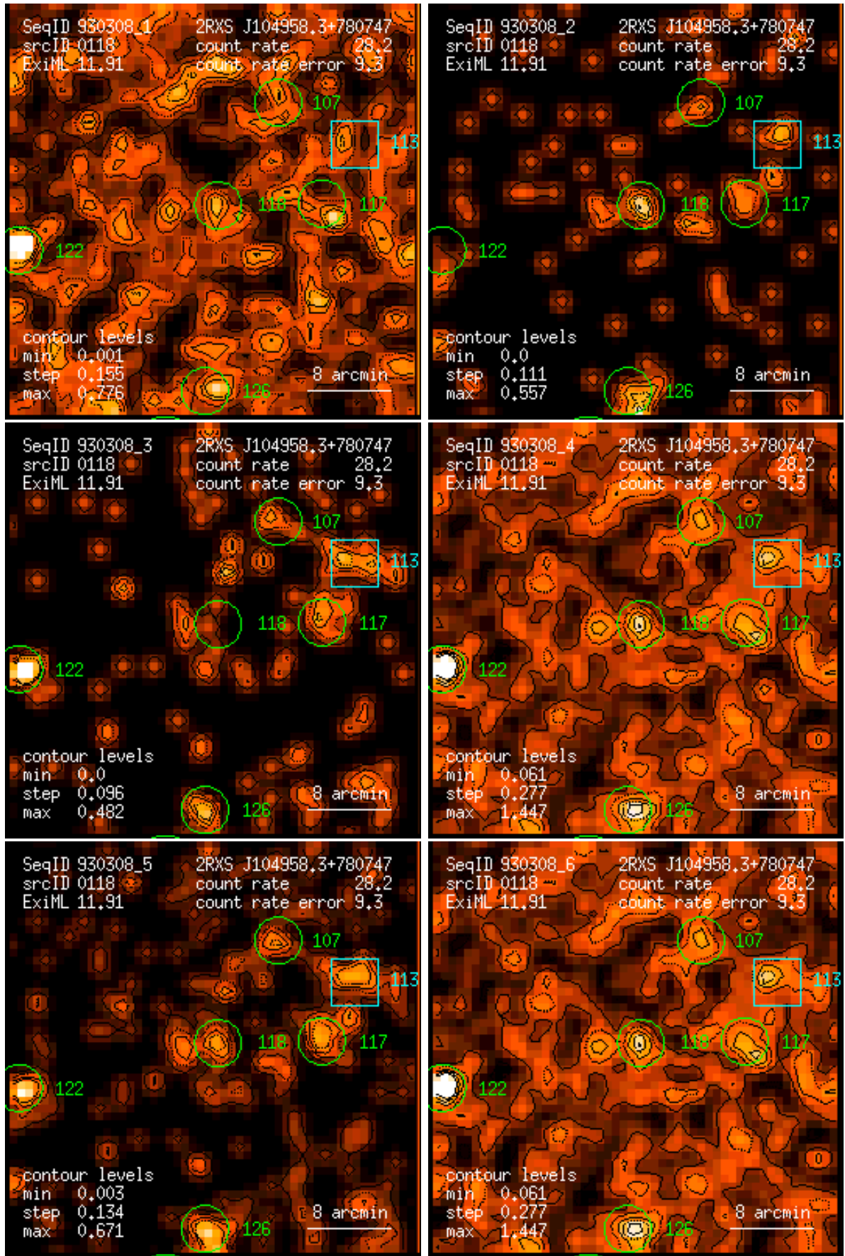
Figure 118: RASS 930308: detection 0118: band rate images, Gaussian filter: (1) PSPC channels 11 – 41, (2) 52 – 90, (3) 91 – 201, (4) 11 – 235, (5) 52 – 201, (6) 11 – 201. Broad band rates in counts/ks. Band rate contour levels in counts/ks/arcmin 2 .
