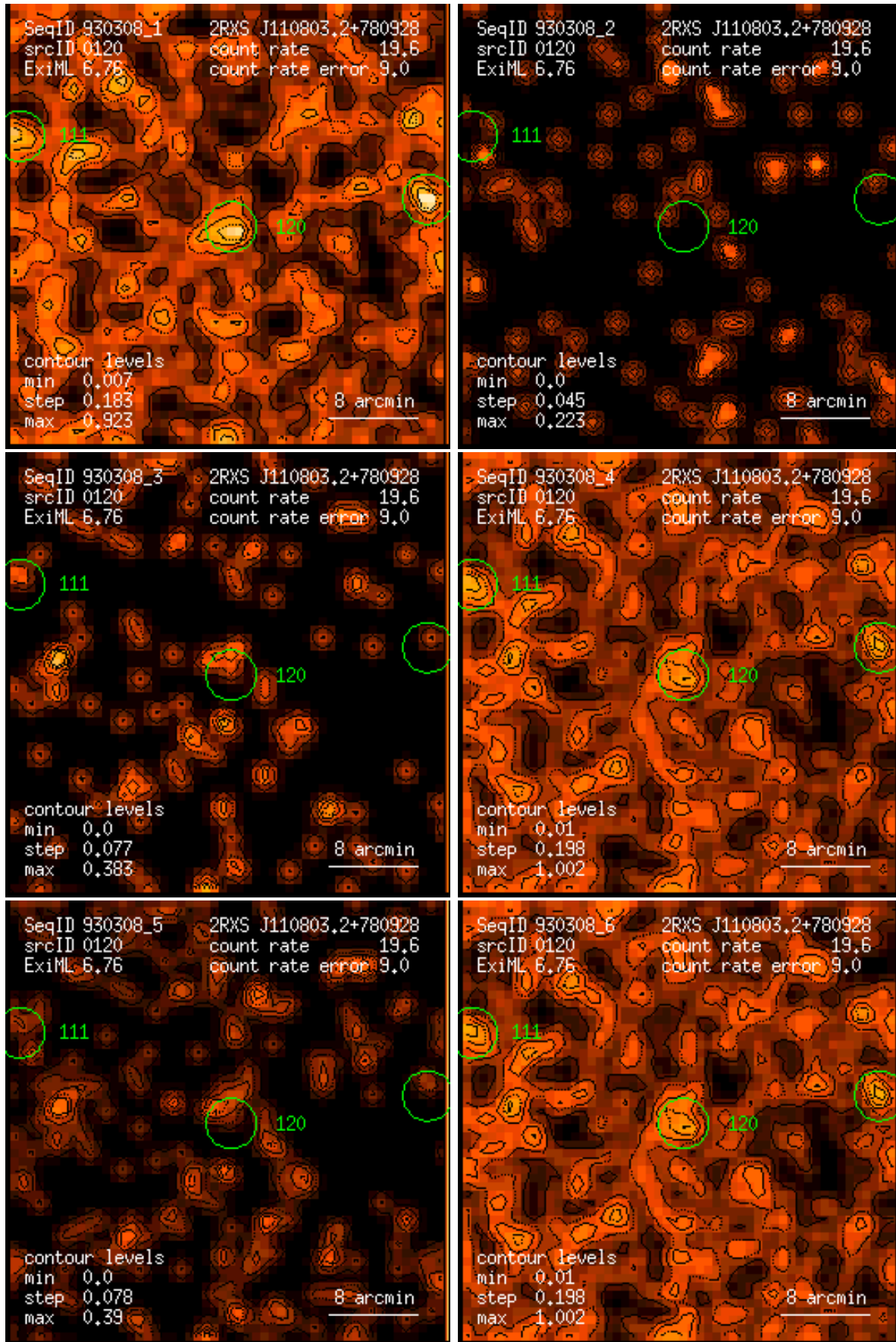
Figure 120: RASS 930308: detection 0120: band rate images, Gaussian filter: (1) PSPC channels 11 – 41, (2) 52 – 90, (3) 91 – 201, (4) 11 – 235, (5) 52 – 201, (6) 11 – 201. Broad band rates in counts/ks. Band rate contour levels in counts/ks/arcmin 2 .
