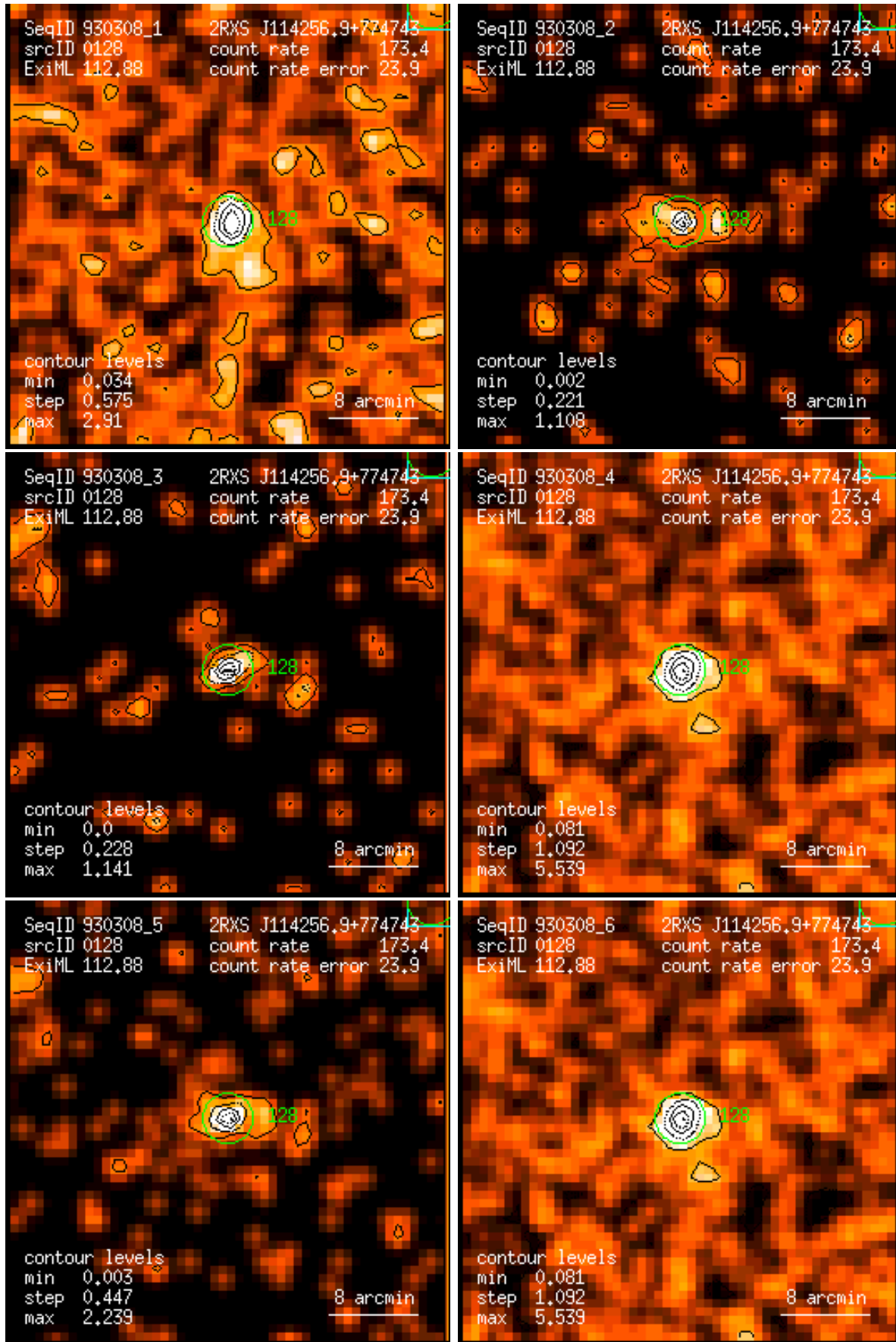
Figure 128: RASS 930308: detection 0128: band rate images, Gaussian filter: (1) PSPC channels 11 – 41, (2) 52 – 90, (3) 91 – 201, (4) 11 – 235, (5) 52 – 201, (6) 11 – 201. Broad band rates in counts/ks. Band rate contour levels in counts/ks/arcmin 2 .
