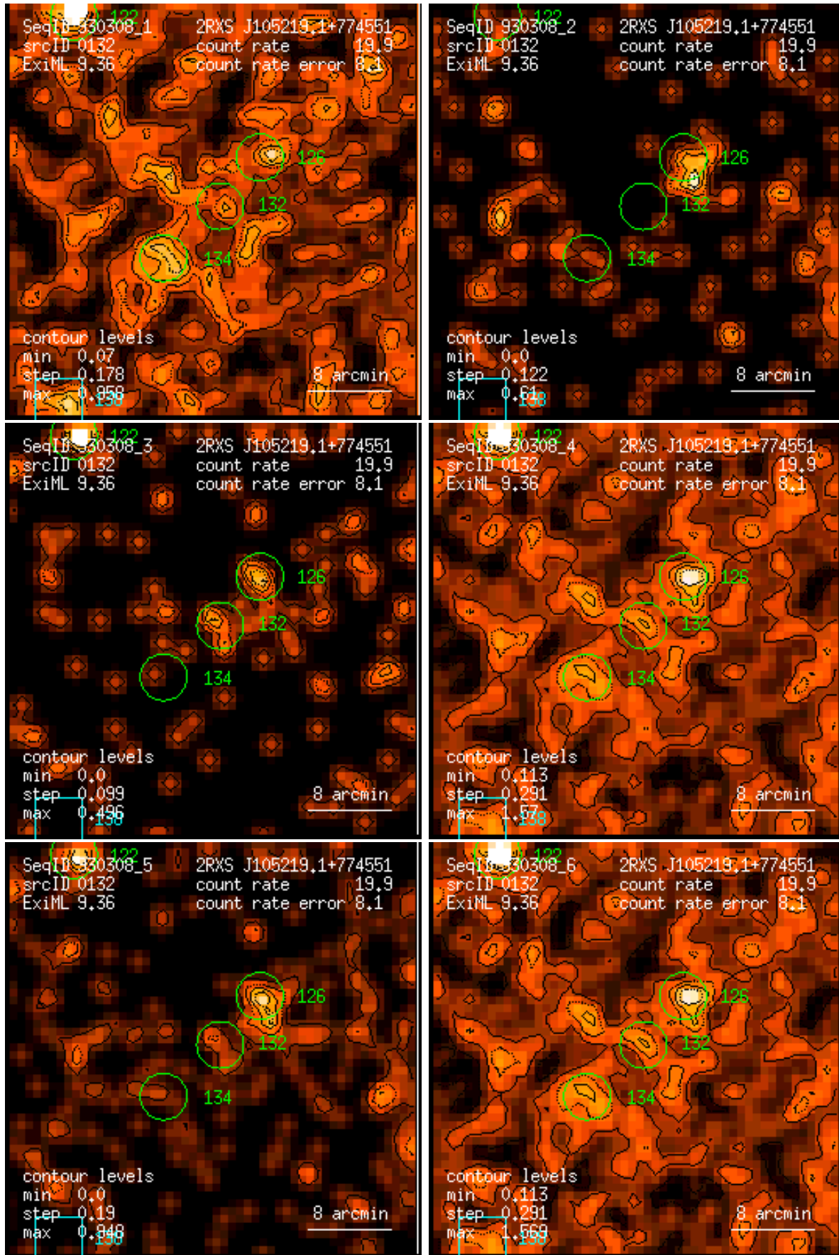
Figure 132: RASS 930308: detection 0132: band rate images, Gaussian filter: (1) PSPC channels 11 – 41, (2) 52 – 90, (3) 91 – 201, (4) 11 – 235, (5) 52 – 201, (6) 11 – 201. Broad band rates in counts/ks. Band rate contour levels in counts/ks/arcmin 2 .
