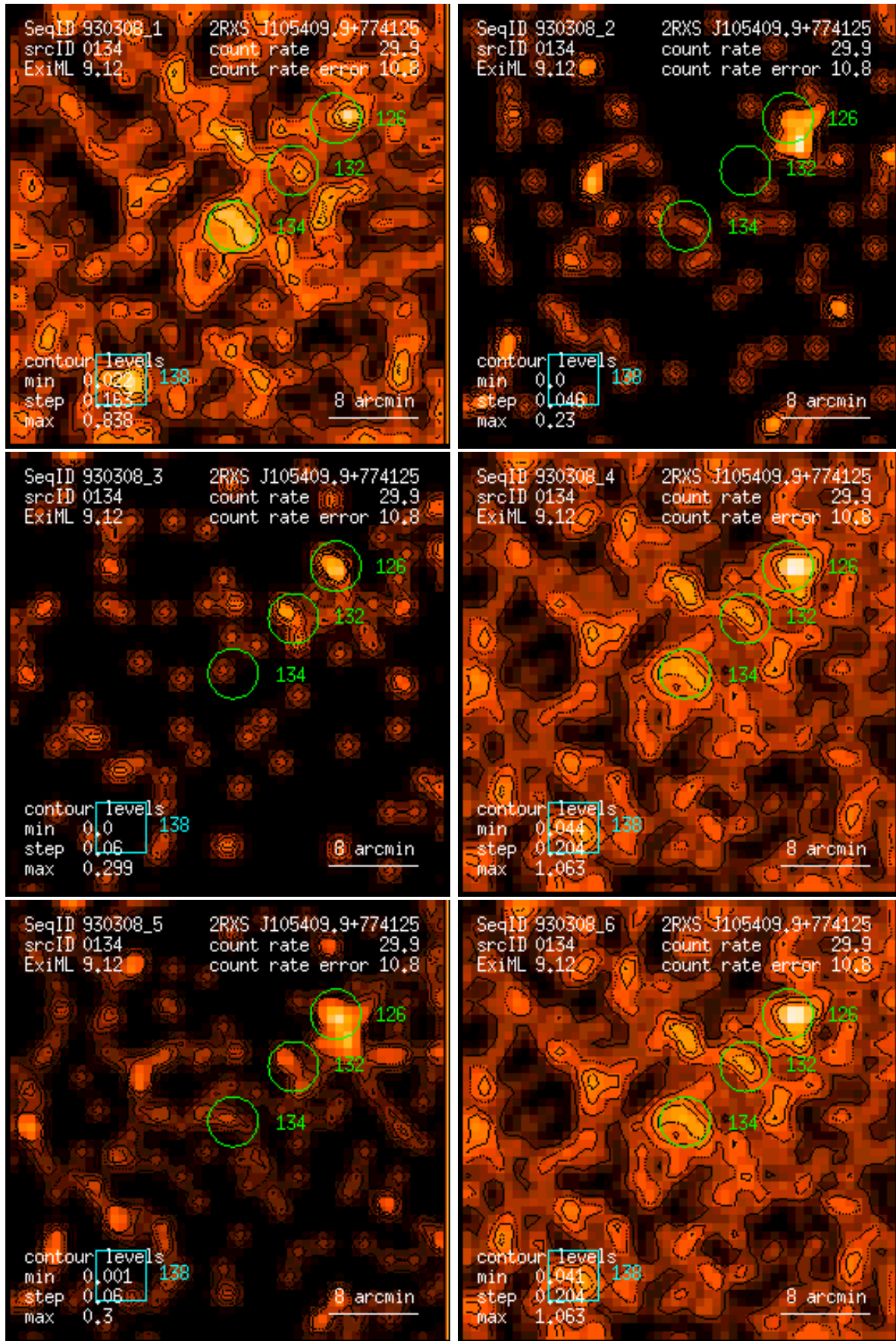
Figure 134: RASS 930308: detection 0134: band rate images, Gaussian filter: (1) PSPC channels 11 – 41, (2) 52 – 90, (3) 91 – 201, (4) 11 – 235, (5) 52 – 201, (6) 11 – 201. Broad band rates in counts/ks. Band rate contour levels in counts/ks/arcmin 2 .
