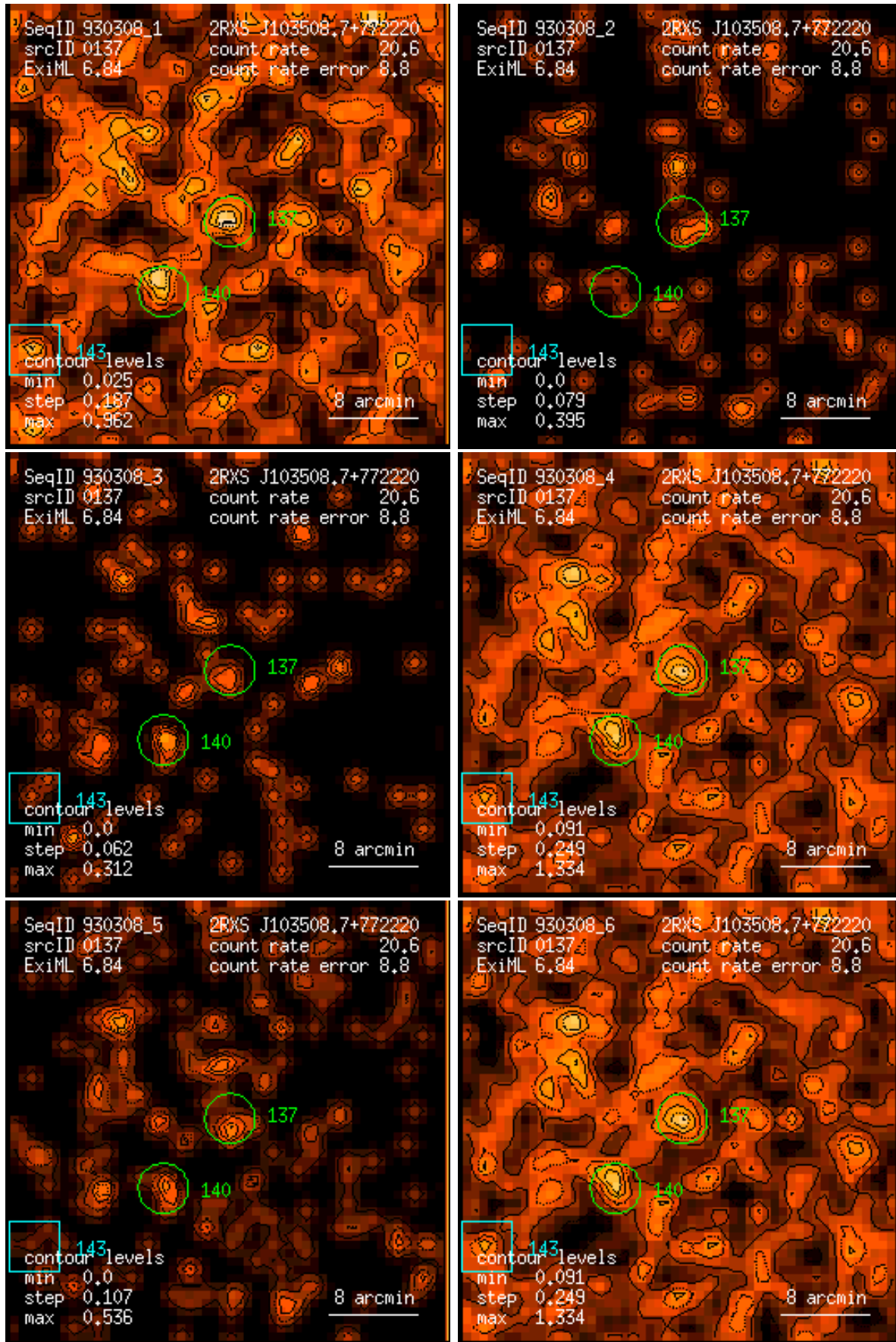
Figure 137: RASS 930308: detection 0137: band rate images, Gaussian filter: (1) PSPC channels 11 – 41, (2) 52 – 90, (3) 91 – 201, (4) 11 – 235, (5) 52 – 201, (6) 11 – 201. Broad band rates in counts/ks. Band rate contour levels in counts/ks/arcmin 2 .
