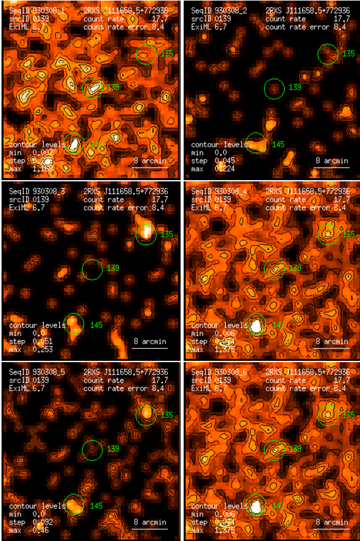
Figure 139: RASS 930308: detection 0139: band rate images, Gaussian filter: (1) PSPC channels 11 – 41, (2) 52 – 90, (3) 91 – 201, (4) 11 – 235, (5) 52 – 201, (6) 11 – 201. Broad band rates in counts/ks. Band rate contour levels in counts/ks/arcmin 2 .
