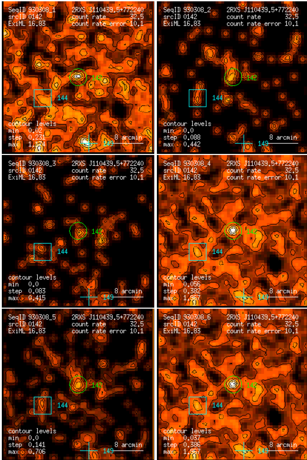
Figure 142: RASS 930308: detection 0142: band rate images, Gaussian filter: (1) PSPC channels 11 – 41, (2) 52 – 90, (3) 91 – 201, (4) 11 – 235, (5) 52 – 201, (6) 11 – 201. Broad band rates in counts/ks. Band rate contour levels in counts/ks/arcmin 2 .
