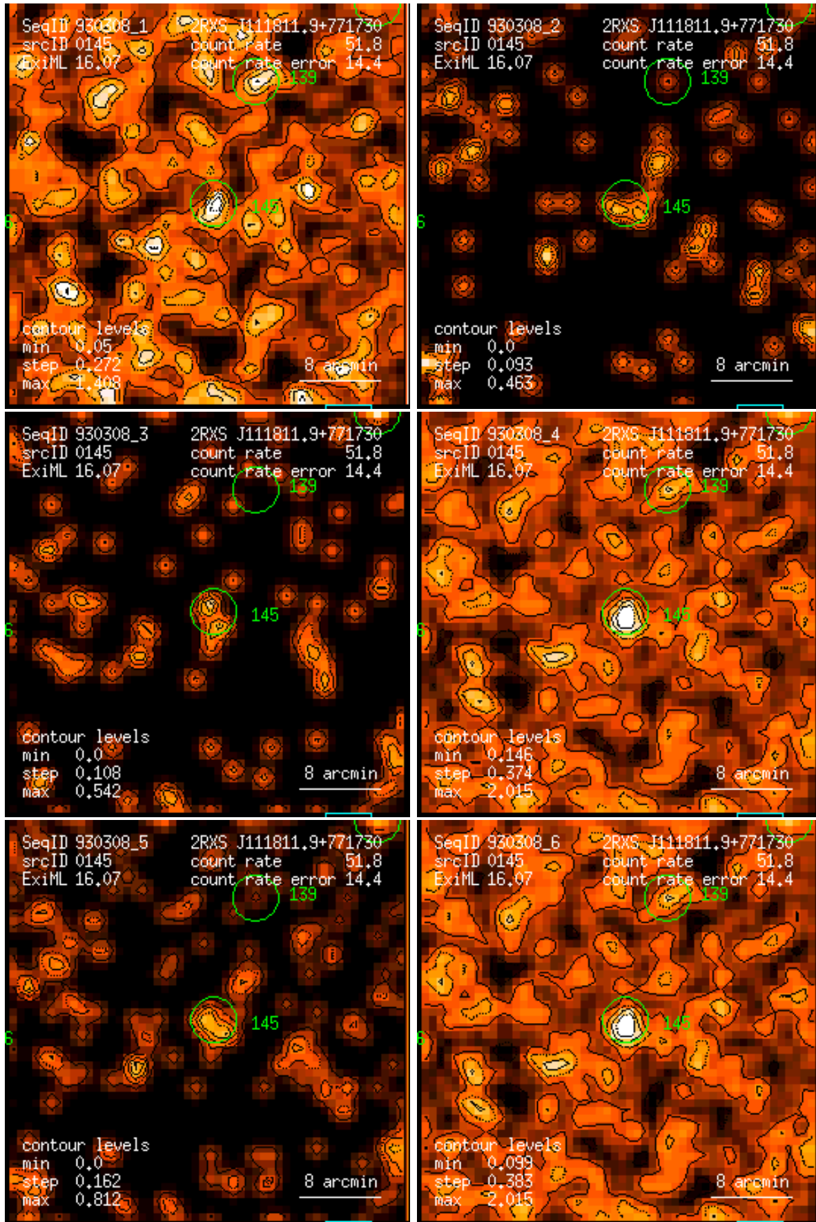
Figure 145: RASS 930308: detection 0145: band rate images, Gaussian filter: (1) PSPC channels 11 – 41, (2) 52 – 90, (3) 91 – 201, (4) 11 – 235, (5) 52 – 201, (6) 11 – 201. Broad band rates in counts/ks. Band rate contour levels in counts/ks/arcmin 2 .
