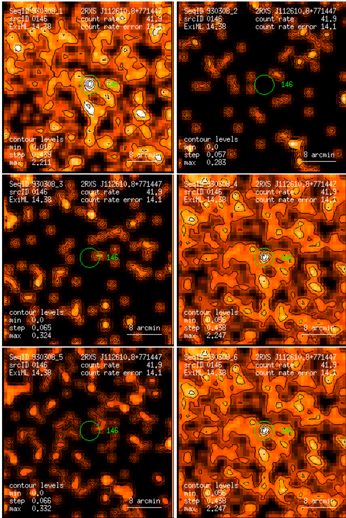
Figure 146: RASS 930308: detection 0146: band rate images, Gaussian filter: (1) PSPC channels 11 – 41, (2) 52 – 90, (3) 91 – 201, (4) 11 – 235, (5) 52 – 201, (6) 11 – 201. Broad band rates in counts/ks. Band rate contour levels in counts/ks/arcmin 2 .
