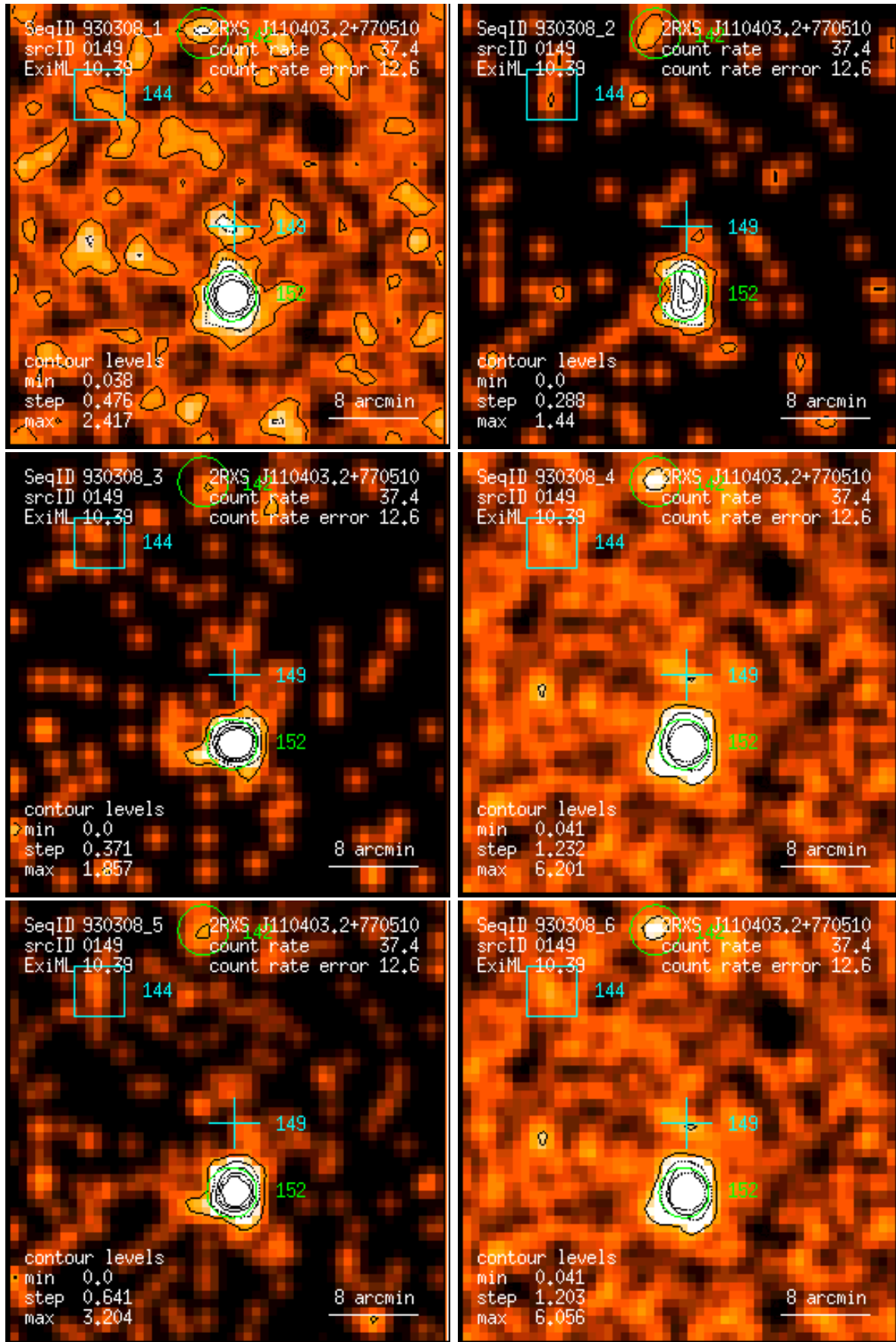
Figure 149: RASS 930308: detection 0149: band rate images, Gaussian filter: (1) PSPC channels 11 – 41, (2) 52 – 90, (3) 91 – 201, (4) 11 – 235, (5) 52 – 201, (6) 11 – 201. Broad band rates in counts/ks. Band rate contour levels in counts/ks/arcmin 2 .
