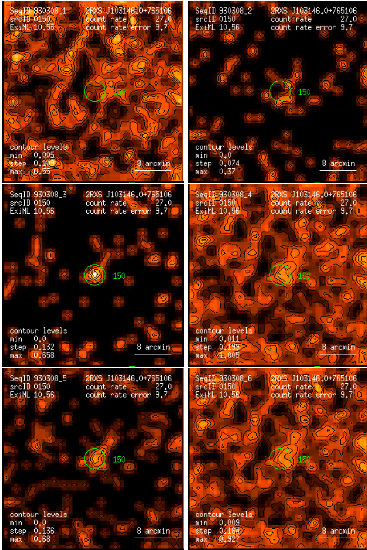
Figure 150: RASS 930308: detection 0150: band rate images, Gaussian filter: (1) PSPC channels 11 – 41, (2) 52 – 90, (3) 91 – 201, (4) 11 – 235, (5) 52 – 201, (6) 11 – 201. Broad band rates in counts/ks. Band rate contour levels in counts/ks/arcmin 2 .
