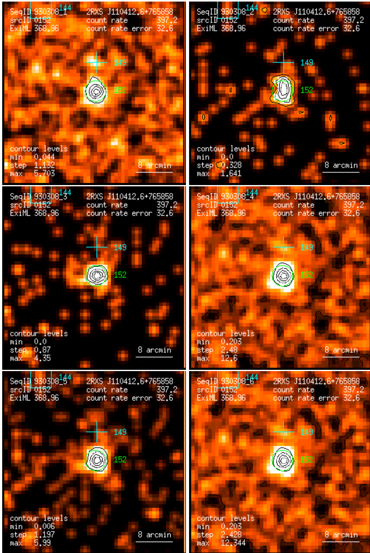
Figure 152: RASS 930308: detection 0152: band rate images, Gaussian filter: (1) PSPC channels 11 – 41, (2) 52 – 90, (3) 91 – 201, (4) 11 – 235, (5) 52 – 201, (6) 11 – 201. Broad band rates in counts/ks. Band rate contour levels in counts/ks/arcmin 2 .
