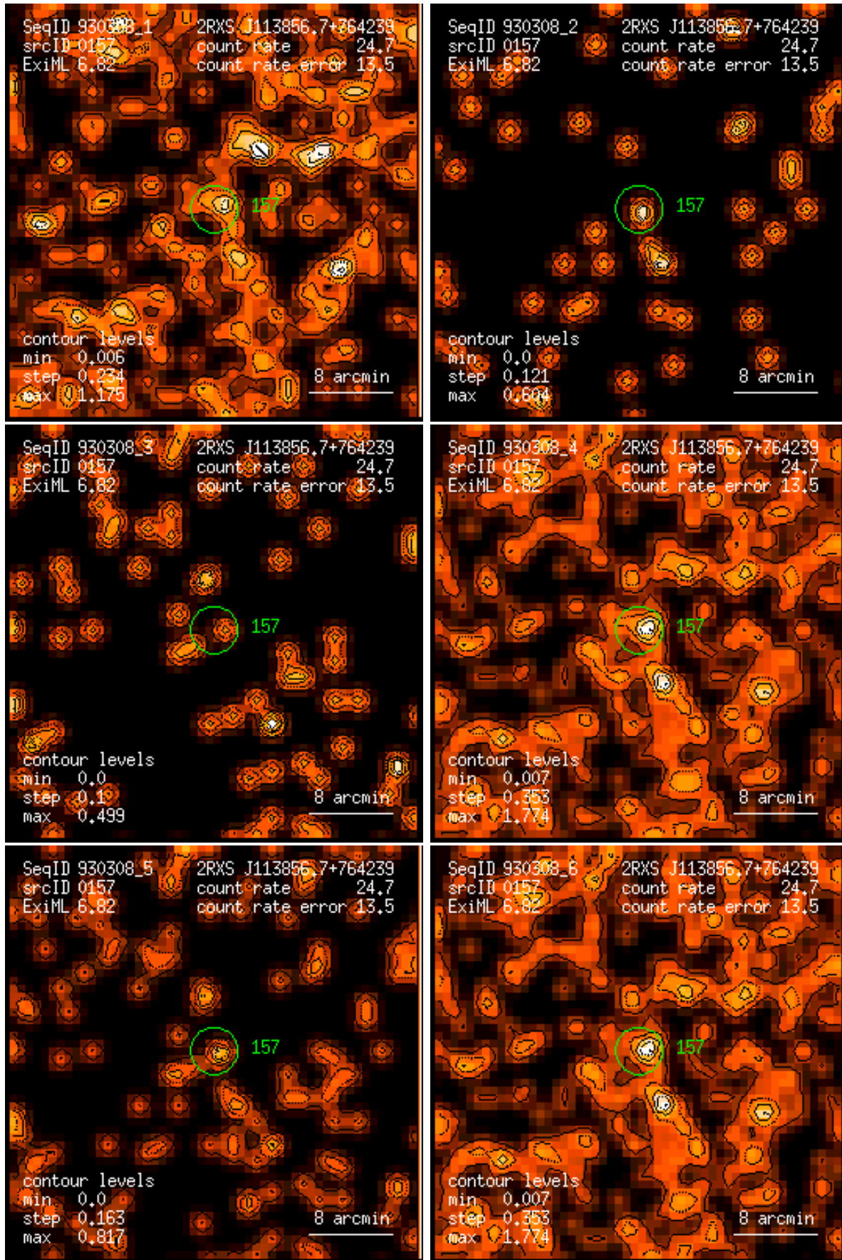
Figure 157: RASS 930308: detection 0157: band rate images, Gaussian filter: (1) PSPC channels 11 – 41, (2) 52 – 90, (3) 91 – 201, (4) 11 – 235, (5) 52 – 201, (6) 11 – 201. Broad band rates in counts/ks. Band rate contour levels in counts/ks/arcmin 2 .
