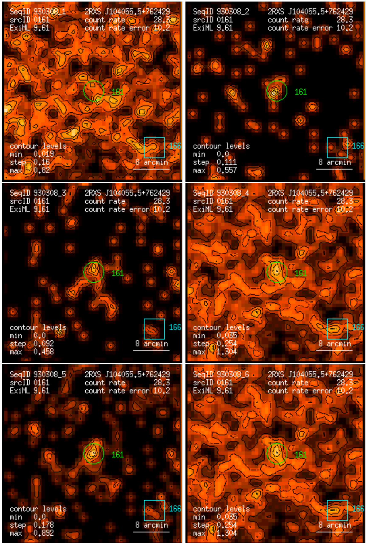
Figure 161: RASS 930308: detection 0161: band rate images, Gaussian filter: (1) PSPC channels 11 – 41, (2) 52 – 90, (3) 91 – 201, (4) 11 – 235, (5) 52 – 201, (6) 11 – 201. Broad band rates in counts/ks. Band rate contour levels in counts/ks/arcmin 2 .
