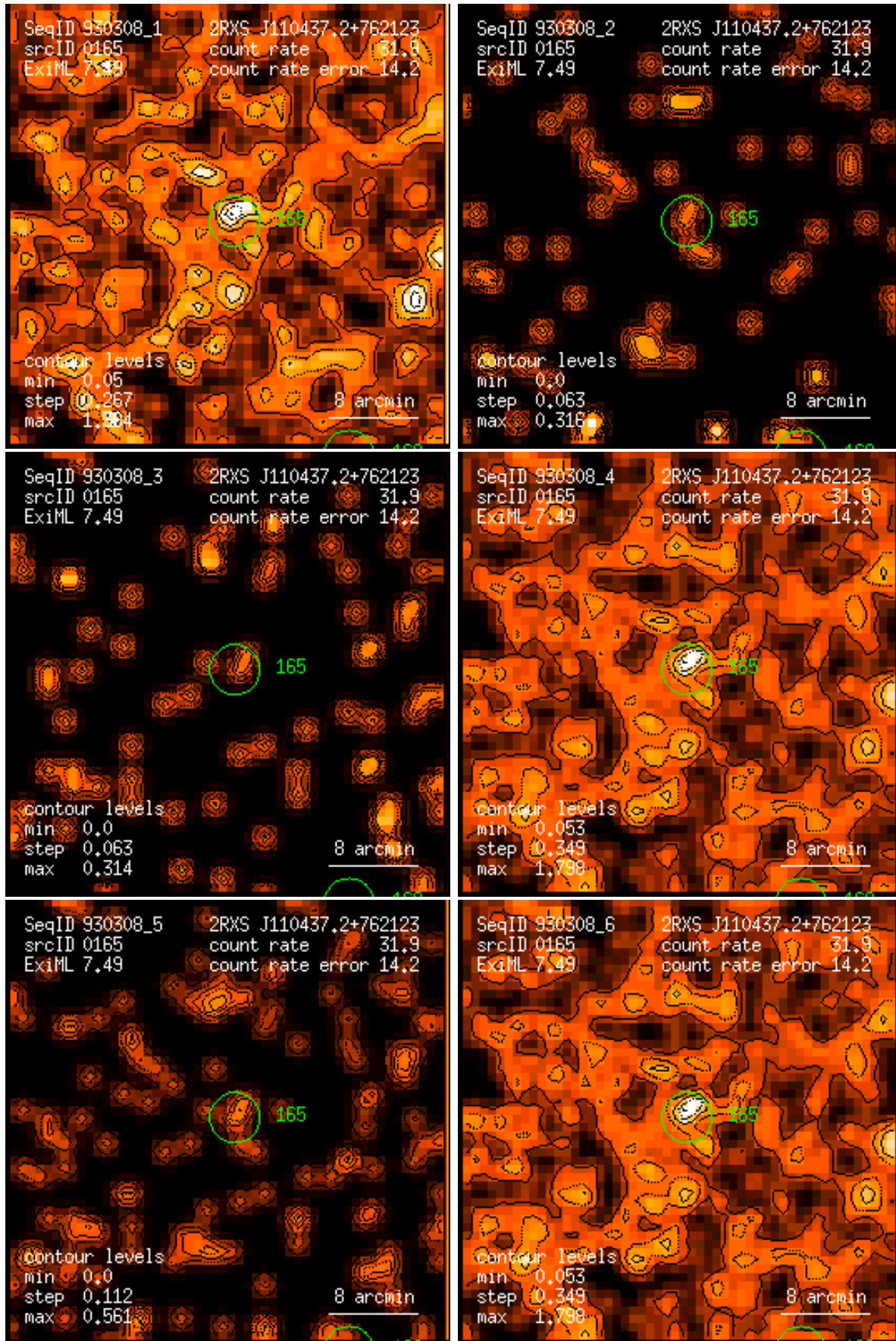
Figure 165: RASS 930308: detection 0165: band rate images, Gaussian filter: (1) PSPC channels 11 – 41, (2) 52 – 90, (3) 91 – 201, (4) 11 – 235, (5) 52 – 201, (6) 11 – 201. Broad band rates in counts/ks. Band rate contour levels in counts/ks/arcmin 2 .
