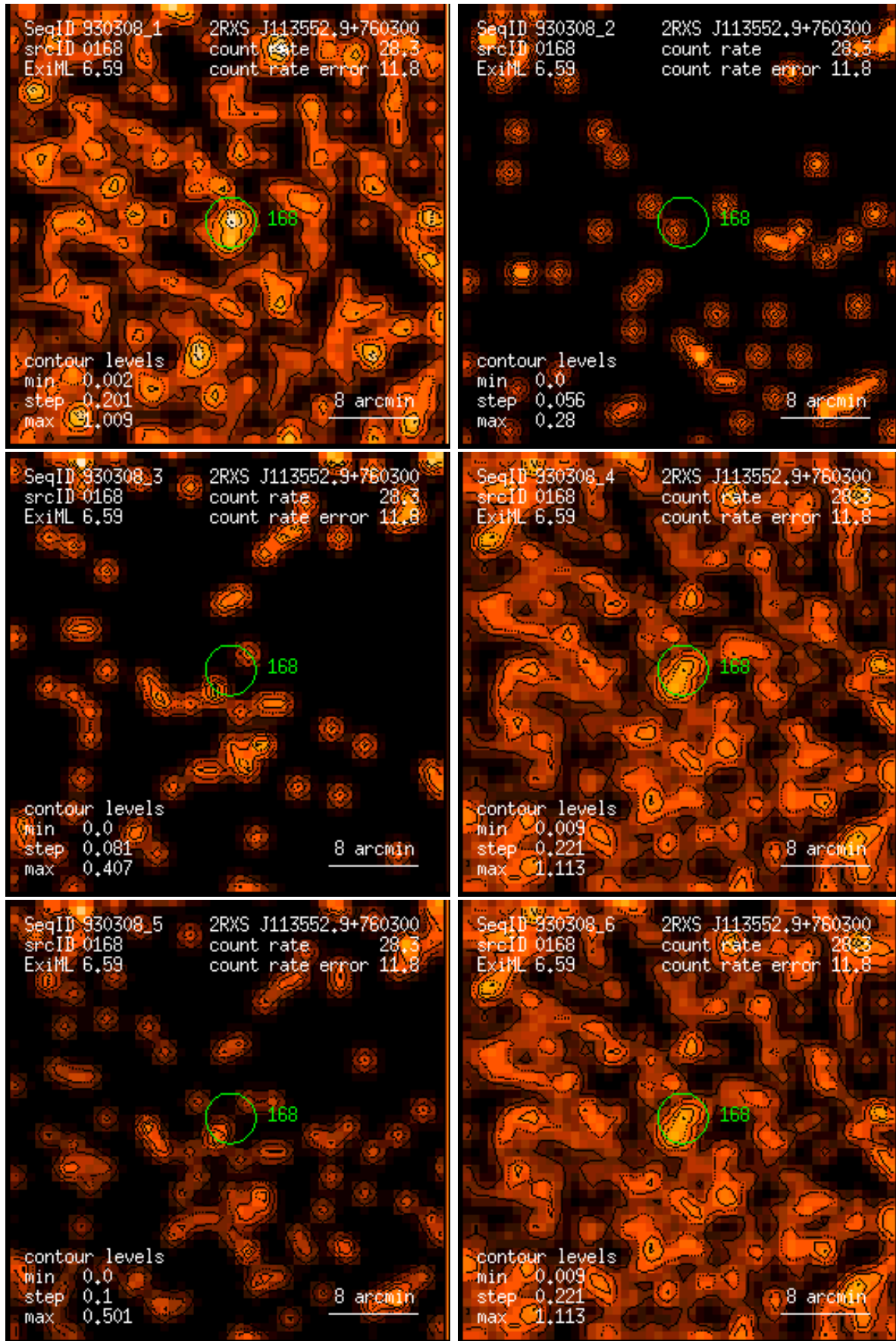
Figure 168: RASS 930308: detection 0168: band rate images, Gaussian filter: (1) PSPC channels 11 – 41, (2) 52 – 90, (3) 91 – 201, (4) 11 – 235, (5) 52 – 201, (6) 11 – 201. Broad band rates in counts/ks. Band rate contour levels in counts/ks/arcmin 2 .
