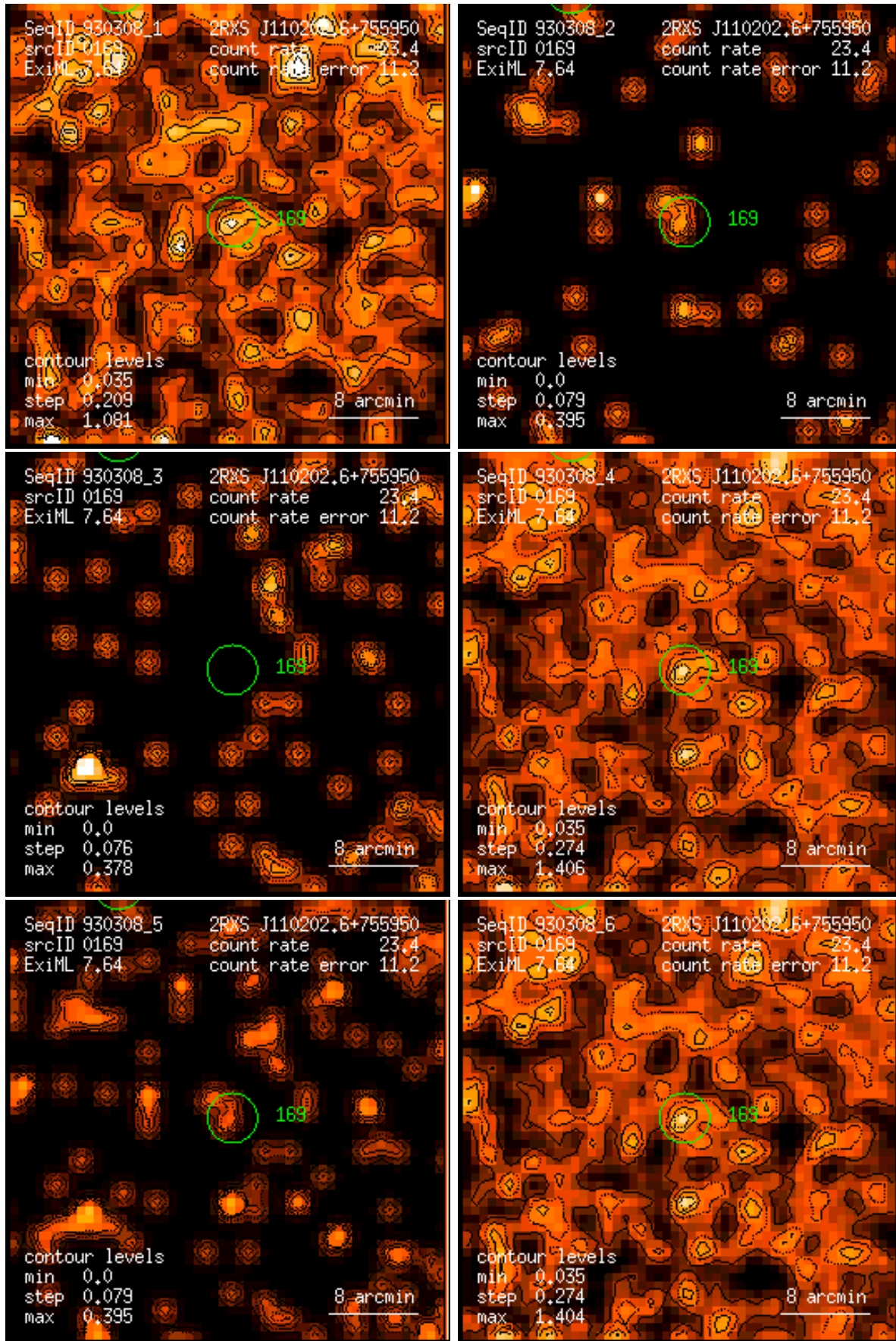
Figure 169: RASS 930308: detection 0169: band rate images, Gaussian filter: (1) PSPC channels 11 – 41, (2) 52 – 90, (3) 91 – 201, (4) 11 – 235, (5) 52 – 201, (6) 11 – 201. Broad band rates in counts/ks. Band rate contour levels in counts/ks/arcmin 2 .
