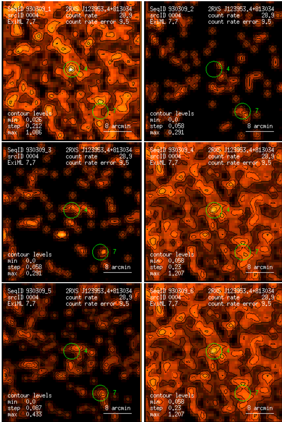
Figure 4: RASS 930309: detection 0004: band rate images, Gaussian filter: (1) PSPC channels 11 – 41, (2) 52 – 90, (3) 91 – 201, (4) 11 – 235, (5) 52 – 201, (6) 11 – 201. Broad band rates in counts/ks. Band rate contour levels in counts/ks/arcmin 2 .
