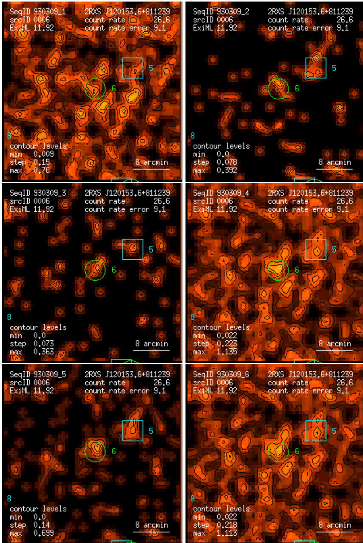
Figure 6: RASS 930309: detection 0006: band rate images, Gaussian filter: (1) PSPC channels 11 – 41, (2) 52 – 90, (3) 91 – 201, (4) 11 – 235, (5) 52 – 201, (6) 11 – 201. Broad band rates in counts/ks. Band rate contour levels in counts/ks/arcmin 2 .
