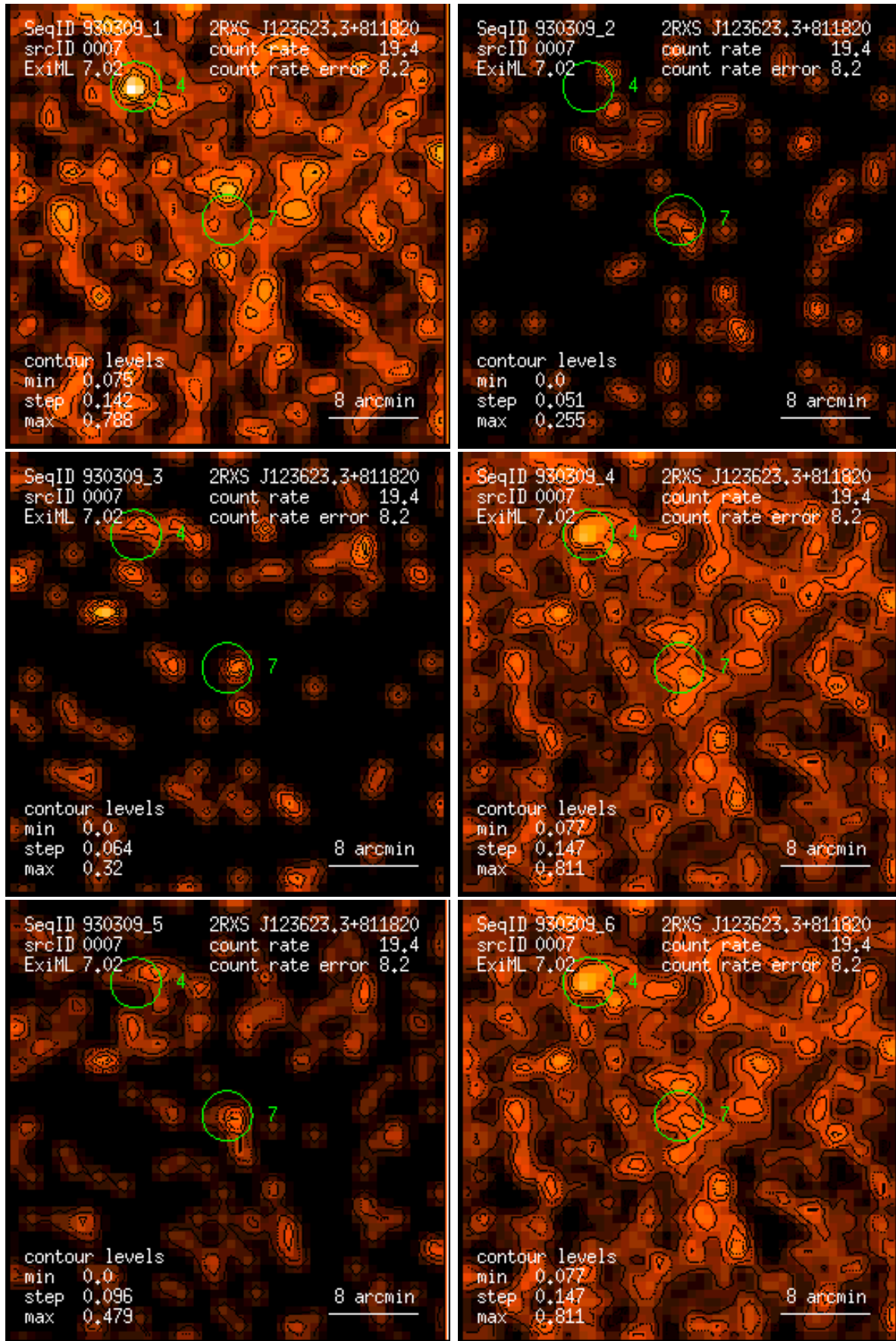
Figure 7: RASS 930309: detection 0007: band rate images, Gaussian filter: (1) PSPC channels 11 – 41, (2) 52 – 90, (3) 91 – 201, (4) 11 – 235, (5) 52 – 201, (6) 11 – 201. Broad band rates in counts/ks. Band rate contour levels in counts/ks/arcmin 2 .
