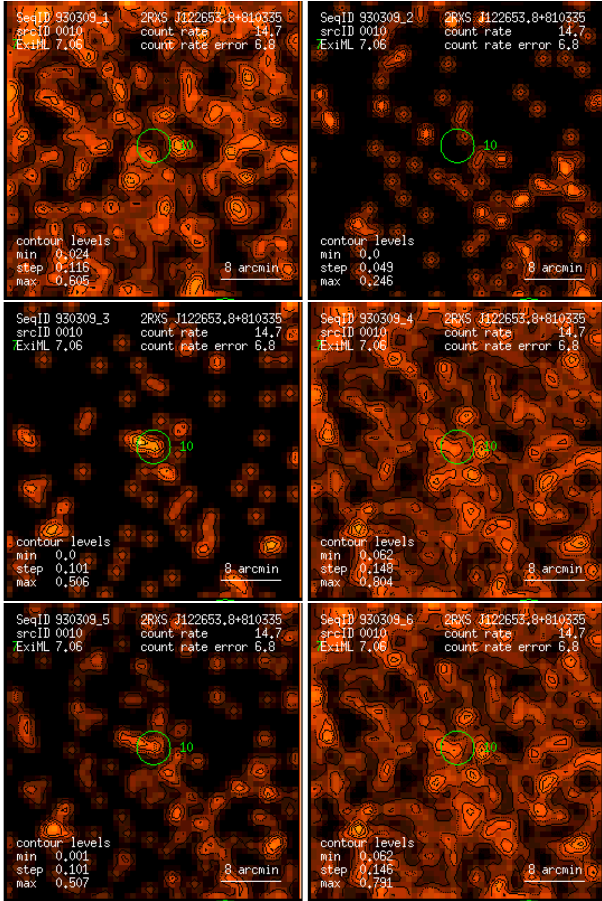
Figure 10: RASS 930309: detection 0010: band rate images, Gaussian filter: (1) PSPC channels 11 – 41, (2) 52 – 90, (3) 91 – 201, (4) 11 – 235, (5) 52 – 201, (6) 11 – 201. Broad band rates in counts/ks. Band rate contour levels in counts/ks/arcmin 2 .
