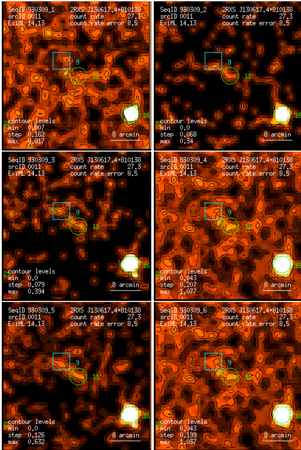
Figure 11: RASS 930309: detection 0011: band rate images, Gaussian filter: (1) PSPC channels 11 – 41, (2) 52 – 90, (3) 91 – 201, (4) 11 – 235, (5) 52 – 201, (6) 11 – 201. Broad band rates in counts/ks. Band rate contour levels in counts/ks/arcmin 2 .
