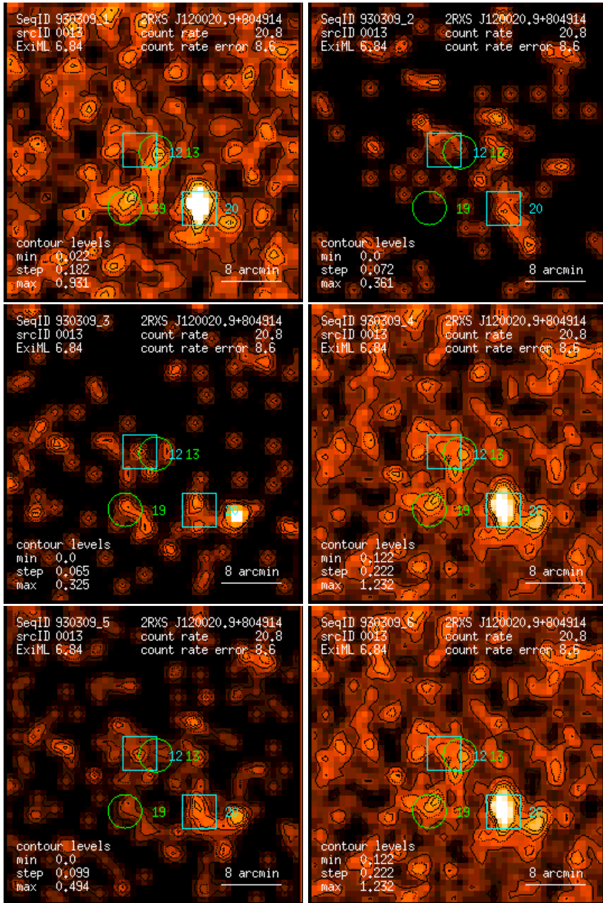
Figure 13: RASS 930309: detection 0013: band rate images, Gaussian filter: (1) PSPC channels 11 – 41, (2) 52 – 90, (3) 91 – 201, (4) 11 – 235, (5) 52 – 201, (6) 11 – 201. Broad band rates in counts/ks. Band rate contour levels in counts/ks/arcmin 2 .
