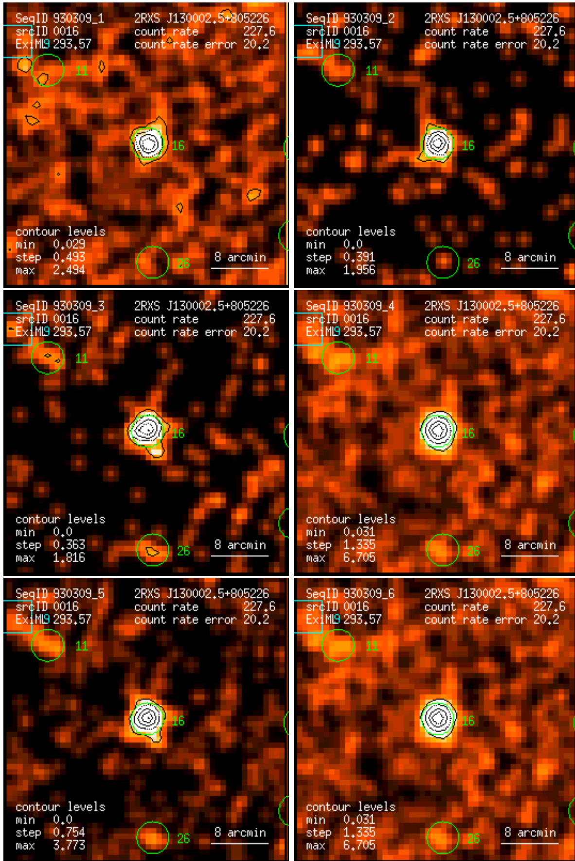
Figure 16: RASS 930309: detection 0016: band rate images, Gaussian filter: (1) PSPC channels 11 – 41, (2) 52 – 90, (3) 91 – 201, (4) 11 – 235, (5) 52 – 201, (6) 11 – 201. Broad band rates in counts/ks. Band rate contour levels in counts/ks/arcmin 2 .
