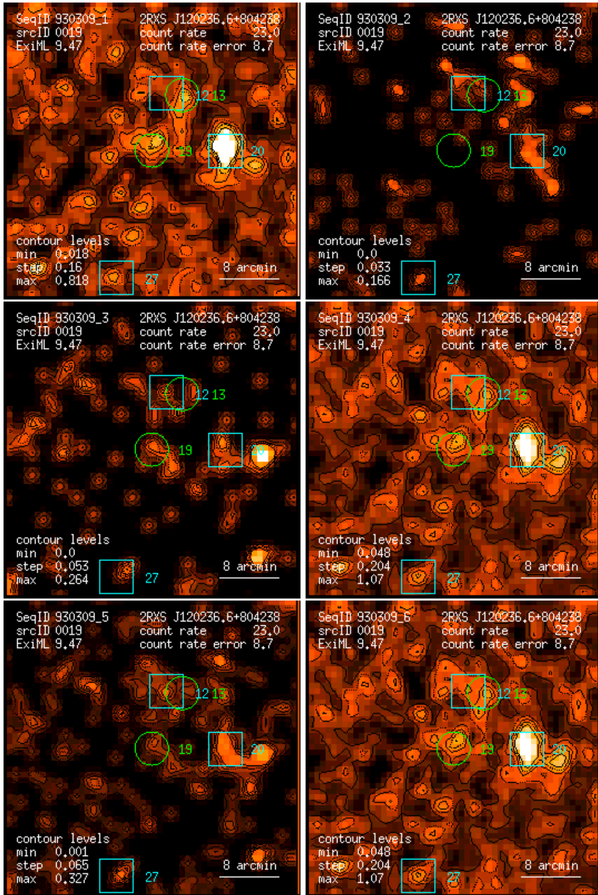
Figure 19: RASS 930309: detection 0019: band rate images, Gaussian filter: (1) PSPC channels 11 – 41, (2) 52 – 90, (3) 91 – 201, (4) 11 – 235, (5) 52 – 201, (6) 11 – 201. Broad band rates in counts/ks. Band rate contour levels in counts/ks/arcmin 2 .
