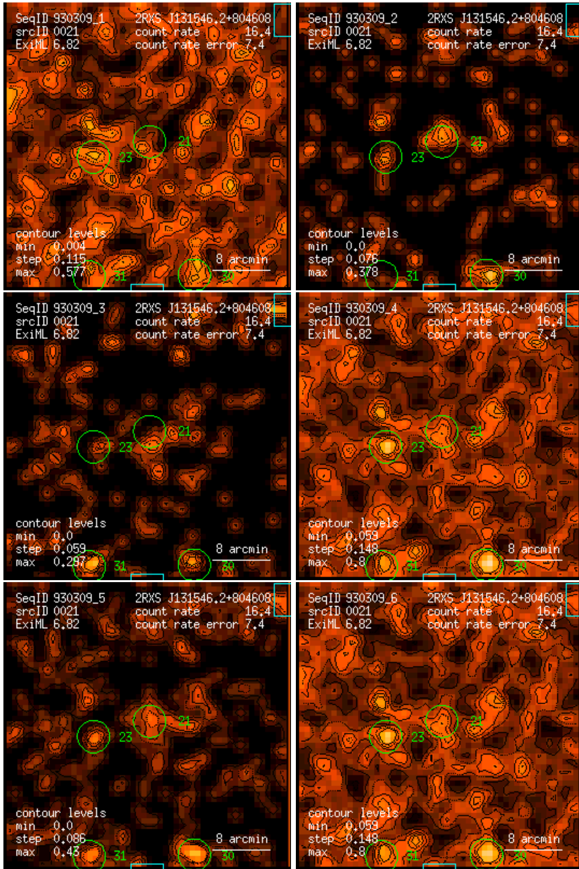
Figure 21: RASS 930309: detection 0021: band rate images, Gaussian filter: (1) PSPC channels 11 – 41, (2) 52 – 90, (3) 91 – 201, (4) 11 – 235, (5) 52 – 201, (6) 11 – 201. Broad band rates in counts/ks. Band rate contour levels in counts/ks/arcmin 2 .
