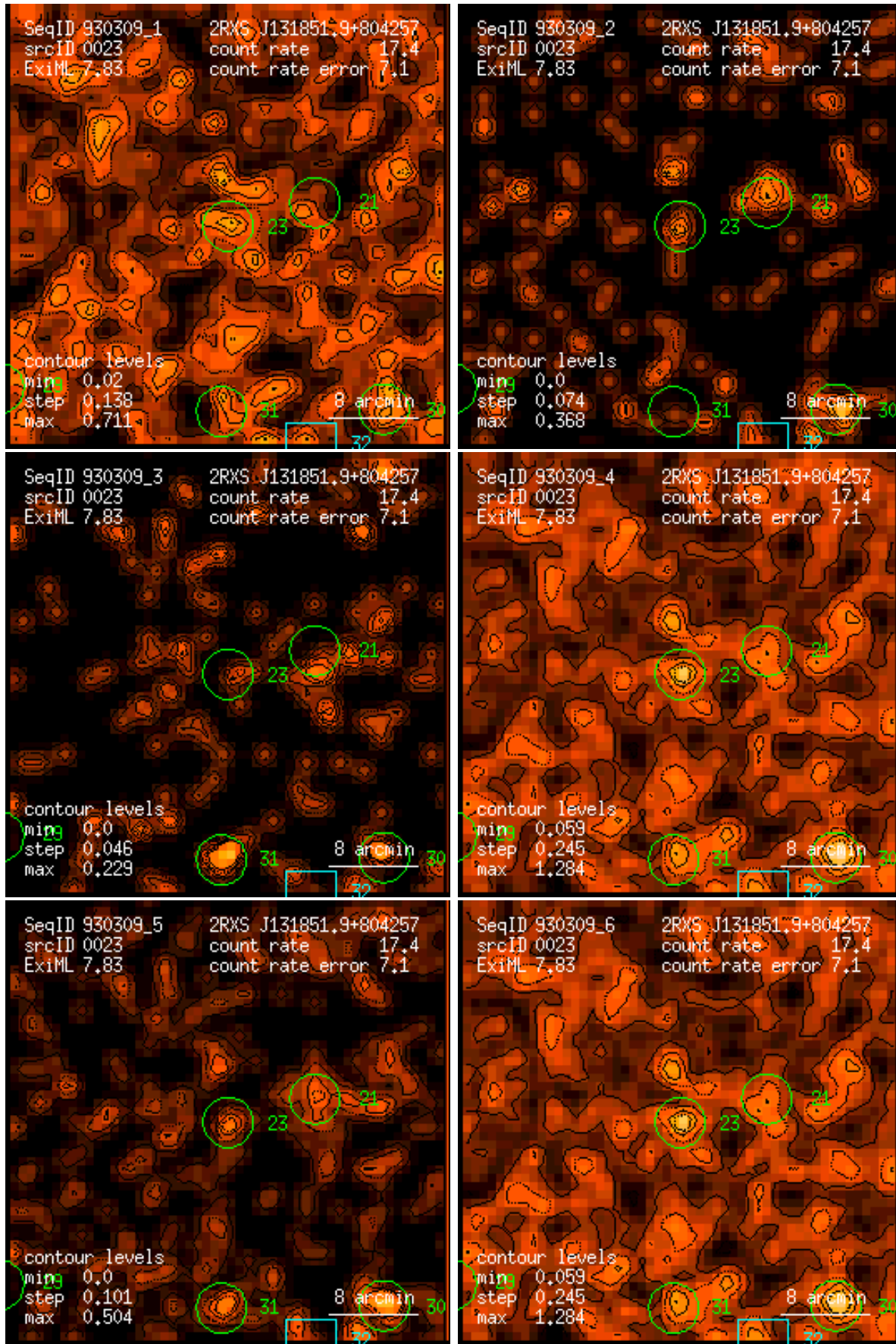
Figure 23: RASS 930309: detection 0023: band rate images, Gaussian filter: (1) PSPC channels 11 – 41, (2) 52 – 90, (3) 91 – 201, (4) 11 – 235, (5) 52 – 201, (6) 11 – 201. Broad band rates in counts/ks. Band rate contour levels in counts/ks/arcmin 2 .
