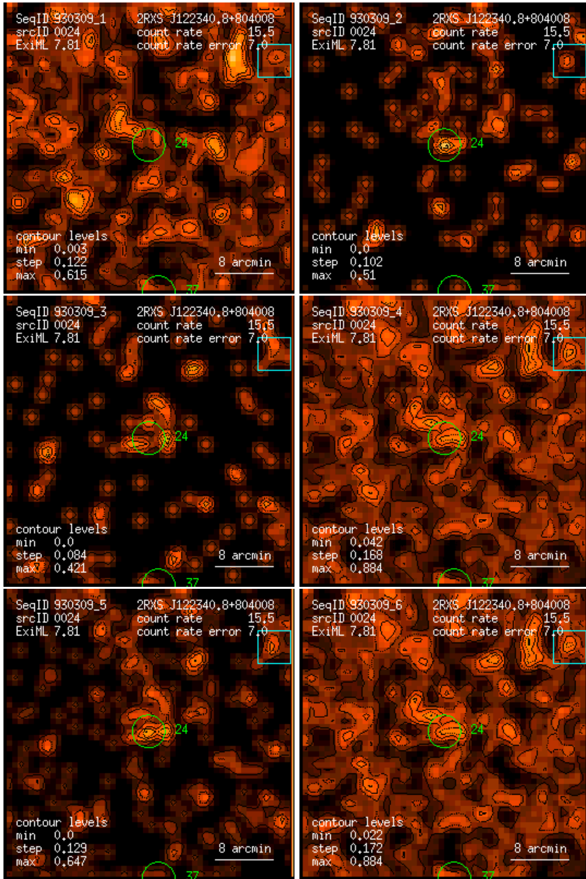
Figure 24: RASS 930309: detection 0024: band rate images, Gaussian filter: (1) PSPC channels 11 – 41, (2) 52 – 90, (3) 91 – 201, (4) 11 – 235, (5) 52 – 201, (6) 11 – 201. Broad band rates in counts/ks. Band rate contour levels in counts/ks/arcmin 2 .
