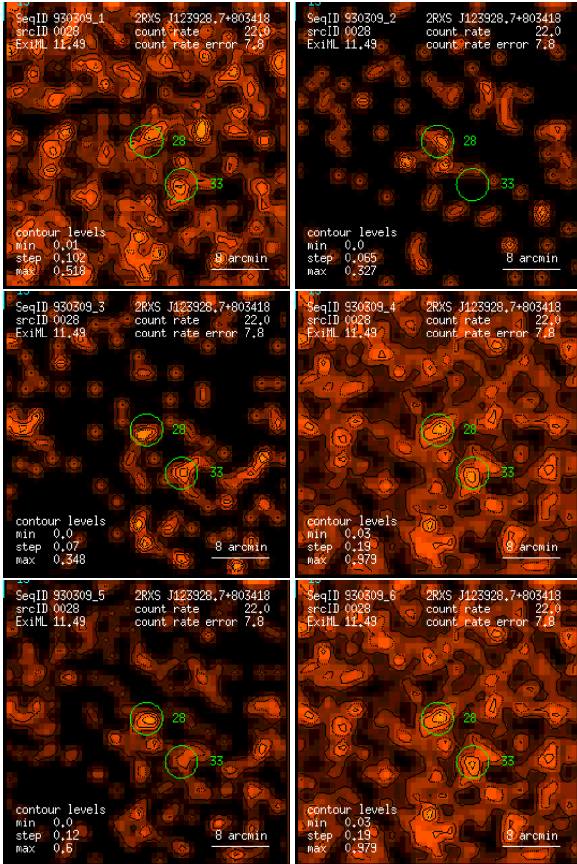
Figure 28: RASS 930309: detection 0028: band rate images, Gaussian filter: (1) PSPC channels 11 – 41, (2) 52 – 90, (3) 91 – 201, (4) 11 – 235, (5) 52 – 201, (6) 11 – 201. Broad band rates in counts/ks. Band rate contour levels in counts/ks/arcmin 2 .
