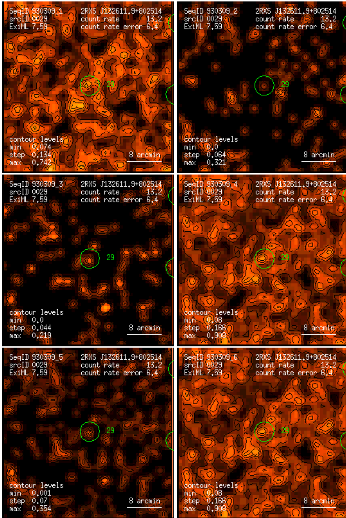
Figure 29: RASS 930309: detection 0029: band rate images, Gaussian filter: (1) PSPC channels 11 – 41, (2) 52 – 90, (3) 91 – 201, (4) 11 – 235, (5) 52 – 201, (6) 11 – 201. Broad band rates in counts/ks. Band rate contour levels in counts/ks/arcmin 2 .
