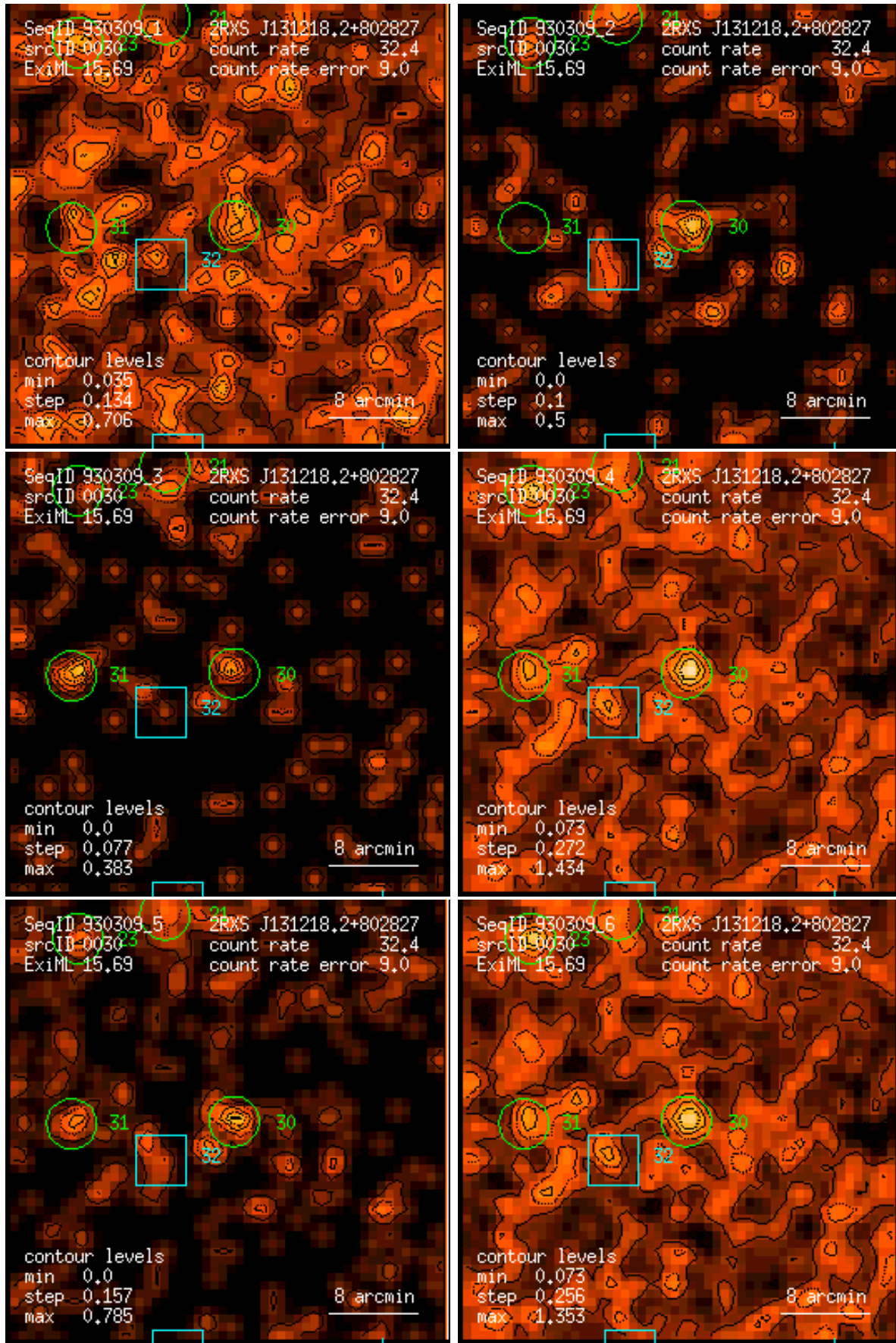
Figure 30: RASS 930309: detection 0030: band rate images, Gaussian filter: (1) PSPC channels 11 – 41, (2) 52 – 90, (3) 91 – 201, (4) 11 – 235, (5) 52 – 201, (6) 11 – 201. Broad band rates in counts/ks. Band rate contour levels in counts/ks/arcmin 2 .
