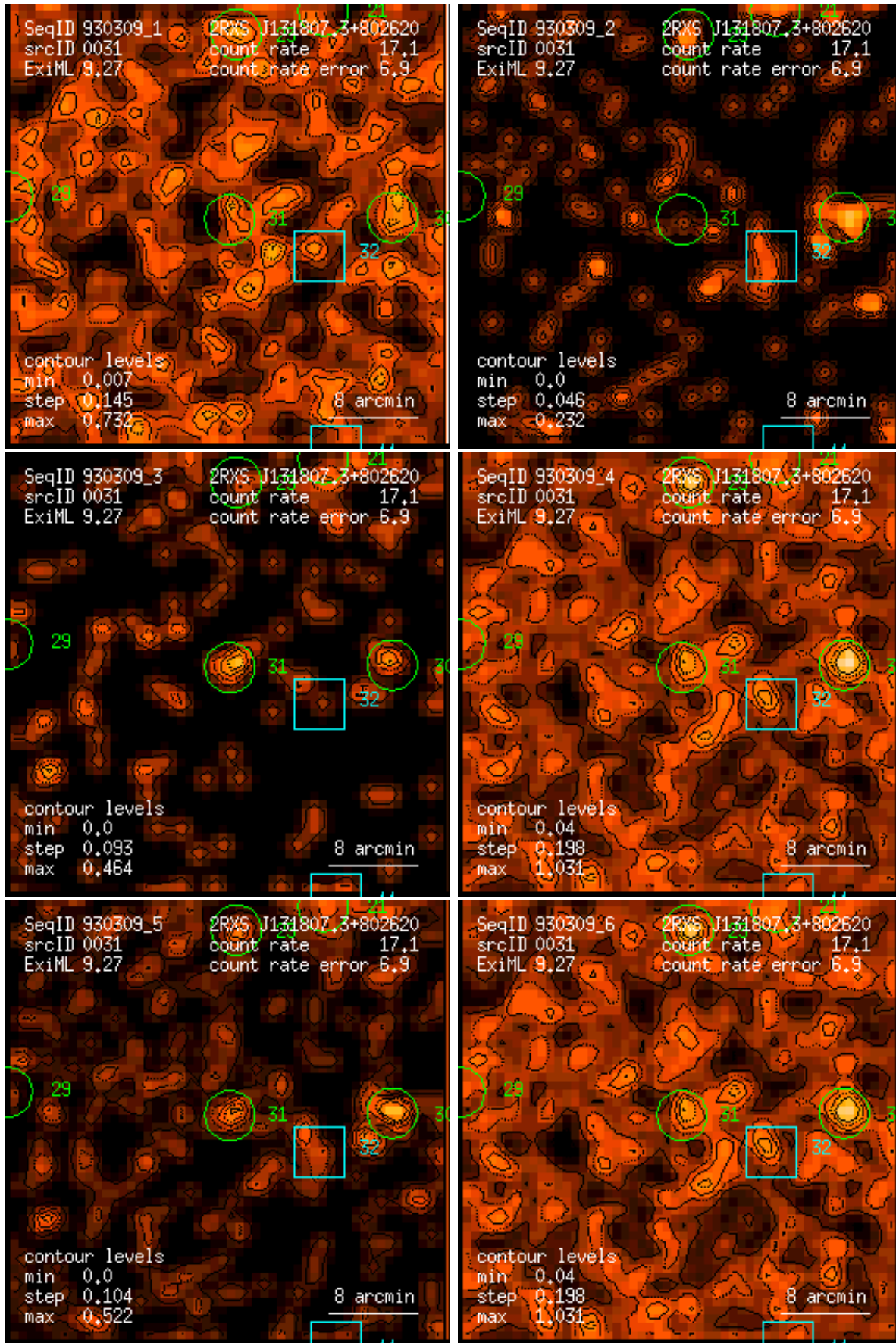
Figure 31: RASS 930309: detection 0031: band rate images, Gaussian filter: (1) PSPC channels 11 – 41, (2) 52 – 90, (3) 91 – 201, (4) 11 – 235, (5) 52 – 201, (6) 11 – 201. Broad band rates in counts/ks. Band rate contour levels in counts/ks/arcmin 2 .
