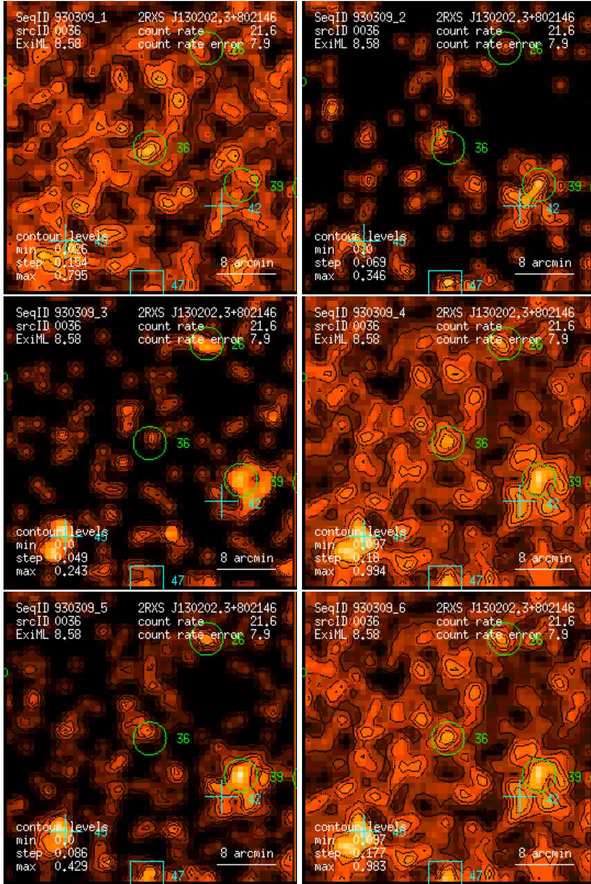
Figure 36: RASS 930309: detection 0036: band rate images, Gaussian filter: (1) PSPC channels 11 – 41, (2) 52 – 90, (3) 91 – 201, (4) 11 – 235, (5) 52 – 201, (6) 11 – 201. Broad band rates in counts/ks. Band rate contour levels in counts/ks/arcmin 2 .
