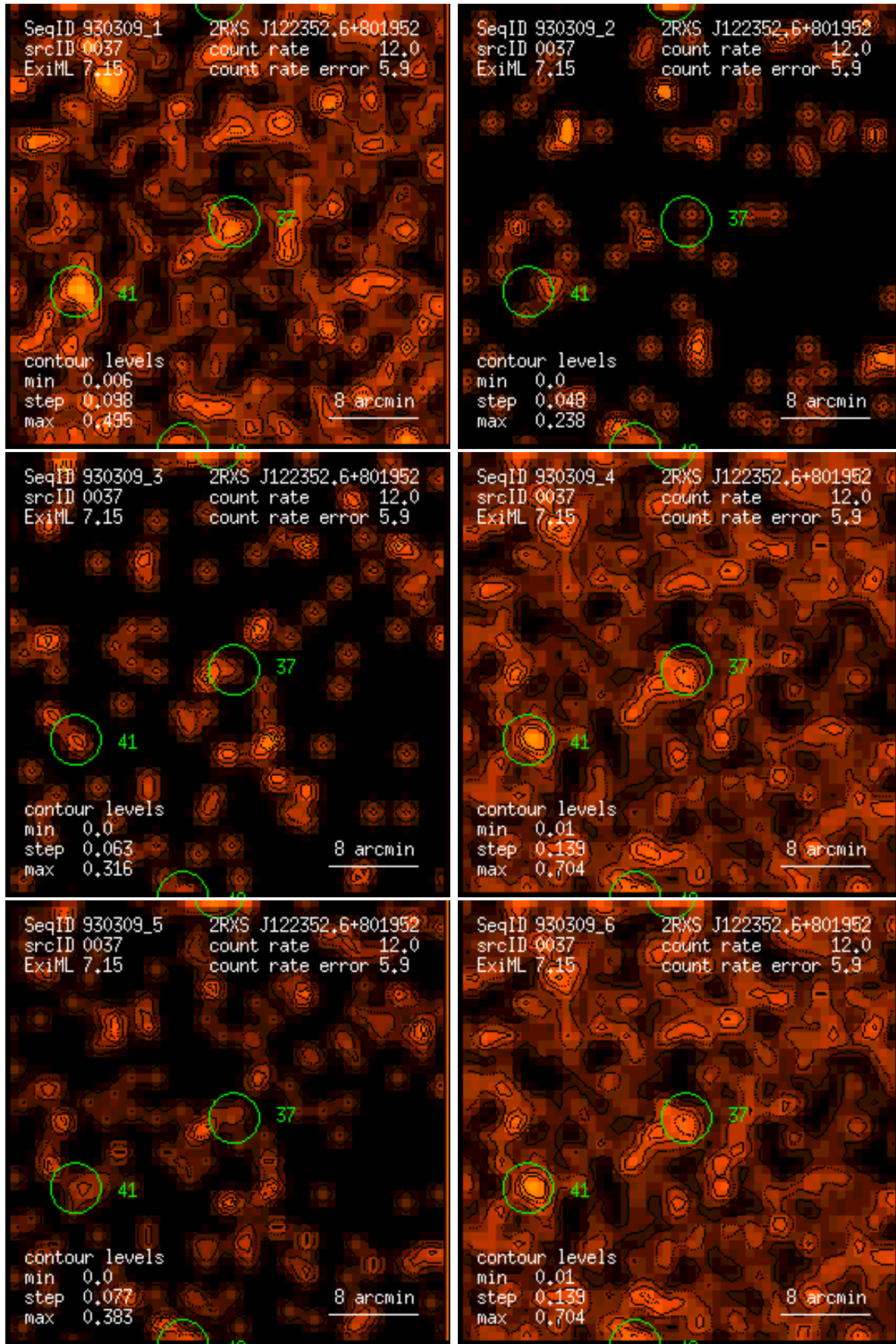
Figure 37: RASS 930309: detection 0037: band rate images, Gaussian filter: (1) PSPC channels 11 – 41, (2) 52 – 90, (3) 91 – 201, (4) 11 – 235, (5) 52 – 201, (6) 11 – 201. Broad band rates in counts/ks. Band rate contour levels in counts/ks/arcmin 2 .
