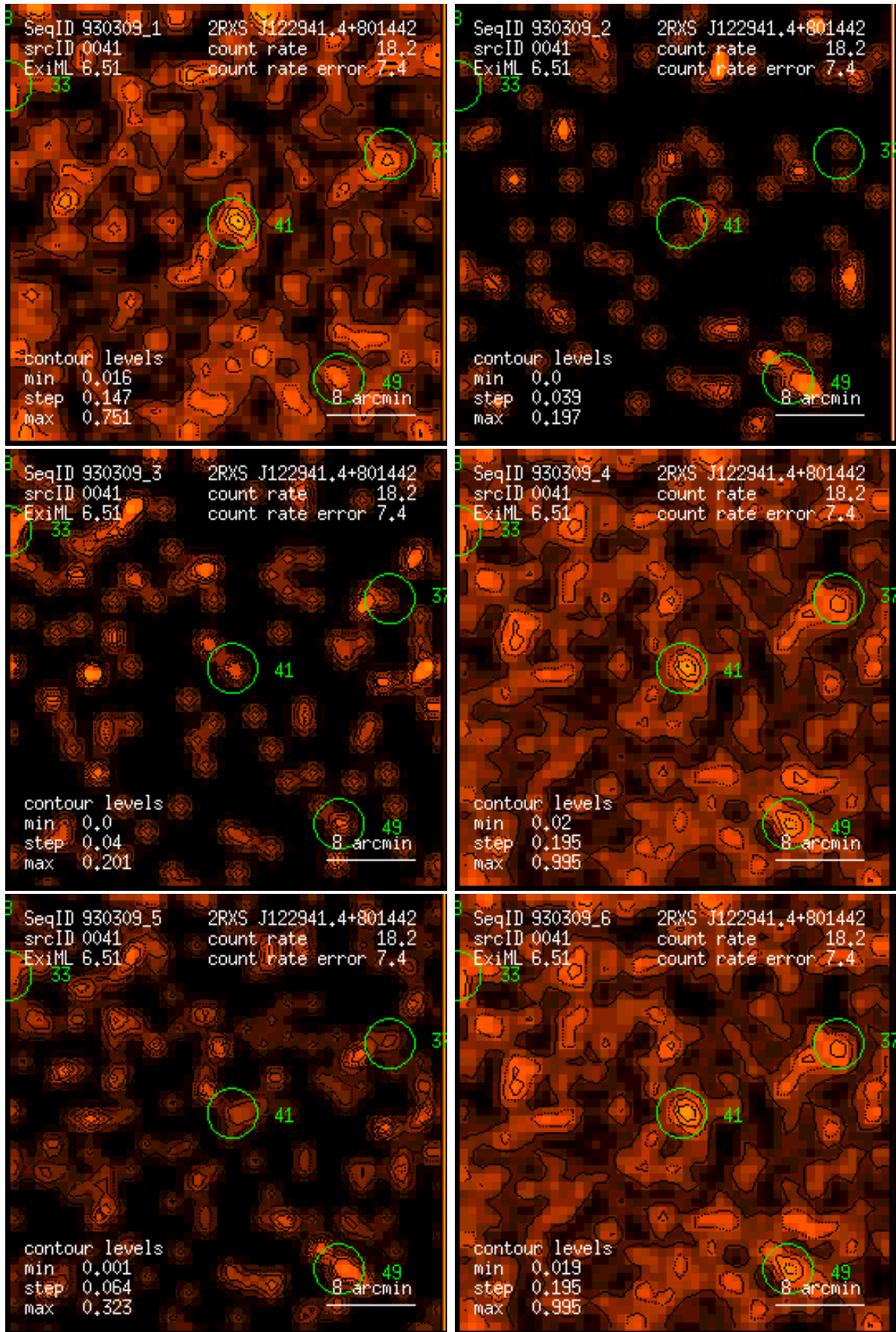
Figure 41: RASS 930309: detection 0041: band rate images, Gaussian filter: (1) PSPC channels 11 – 41, (2) 52 – 90, (3) 91 – 201, (4) 11 – 235, (5) 52 – 201, (6) 11 – 201. Broad band rates in counts/ks. Band rate contour levels in counts/ks/arcmin 2 .
