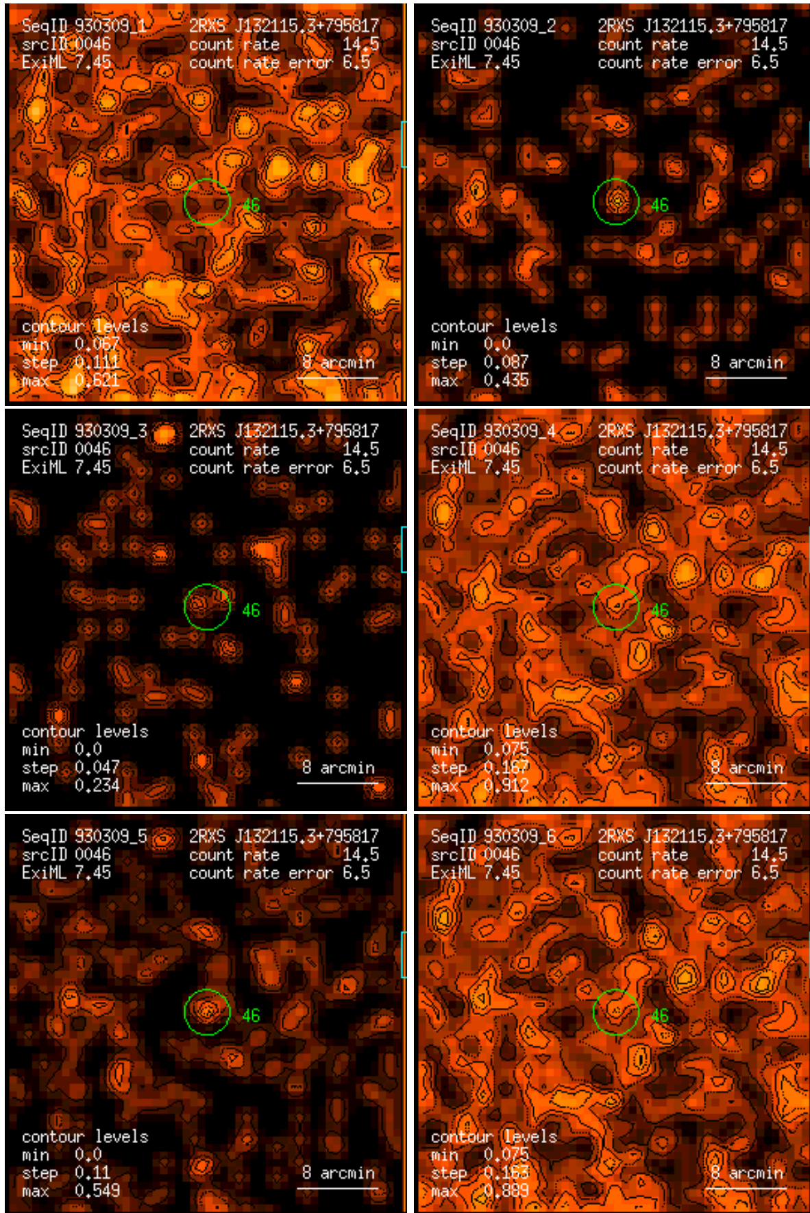
Figure 46: RASS 930309: detection 0046: band rate images, Gaussian filter: (1) PSPC channels 11 – 41, (2) 52 – 90, (3) 91 – 201, (4) 11 – 235, (5) 52 – 201, (6) 11 – 201. Broad band rates in counts/ks. Band rate contour levels in counts/ks/arcmin 2 .
